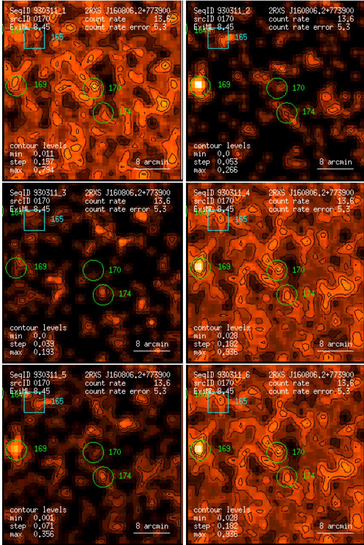
Figure 170: RASS 930311: detection 0170: band rate images, Gaussian filter: (1) PSPC channels 11 – 41, (2) 52 – 90, (3) 91 – 201, (4) 11 – 235, (5) 52 – 201, (6) 11 – 201. Broad band rates in counts/ks. Band rate contour levels in counts/ks/arcmin 2 .
