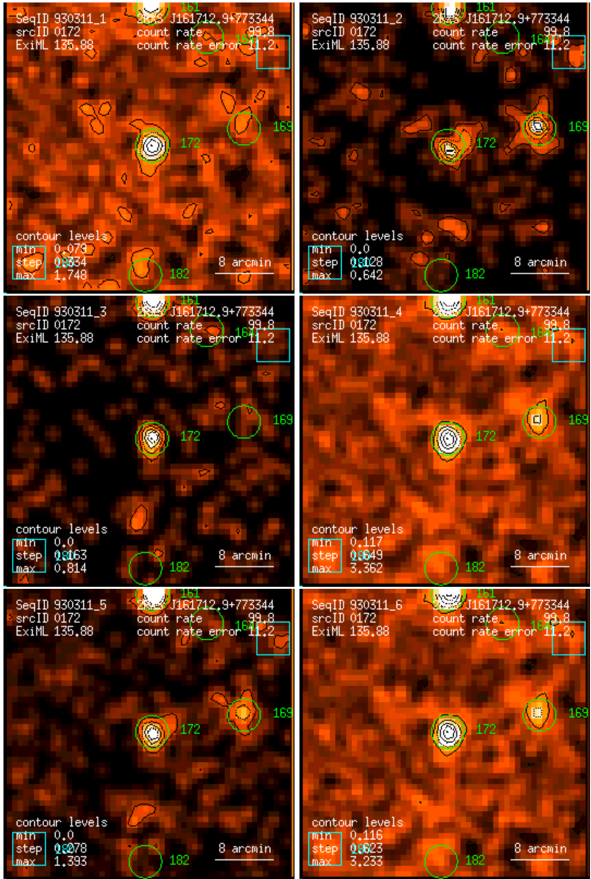
Figure 172: RASS 930311: detection 0172: band rate images, Gaussian filter: (1) PSPC channels 11 – 41, (2) 52 – 90, (3) 91 – 201, (4) 11 – 235, (5) 52 – 201, (6) 11 – 201. Broad band rates in counts/ks. Band rate contour levels in counts/ks/arcmin 2 .
