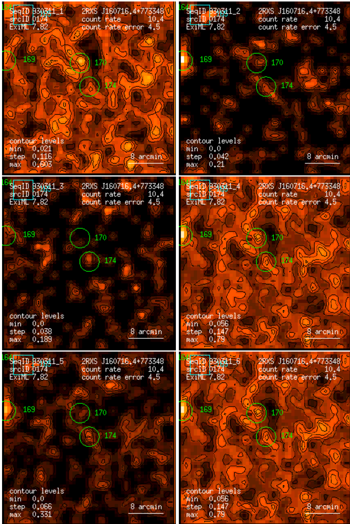
Figure 174: RASS 930311: detection 0174: band rate images, Gaussian filter: (1) PSPC channels 11 – 41, (2) 52 – 90, (3) 91 – 201, (4) 11 – 235, (5) 52 – 201, (6) 11 – 201. Broad band rates in counts/ks. Band rate contour levels in counts/ks/arcmin 2 .
