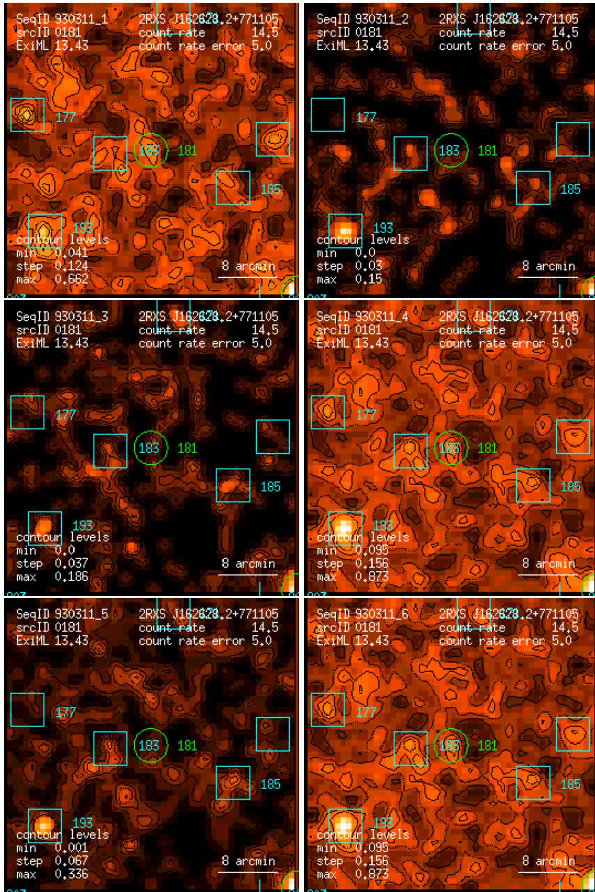
Figure 181: RASS 930311: detection 0181: band rate images, Gaussian filter: (1) PSPC channels 11 – 41, (2) 52 – 90, (3) 91 – 201, (4) 11 – 235, (5) 52 – 201, (6) 11 – 201. Broad band rates in counts/ks. Band rate contour levels in counts/ks/arcmin 2 .
