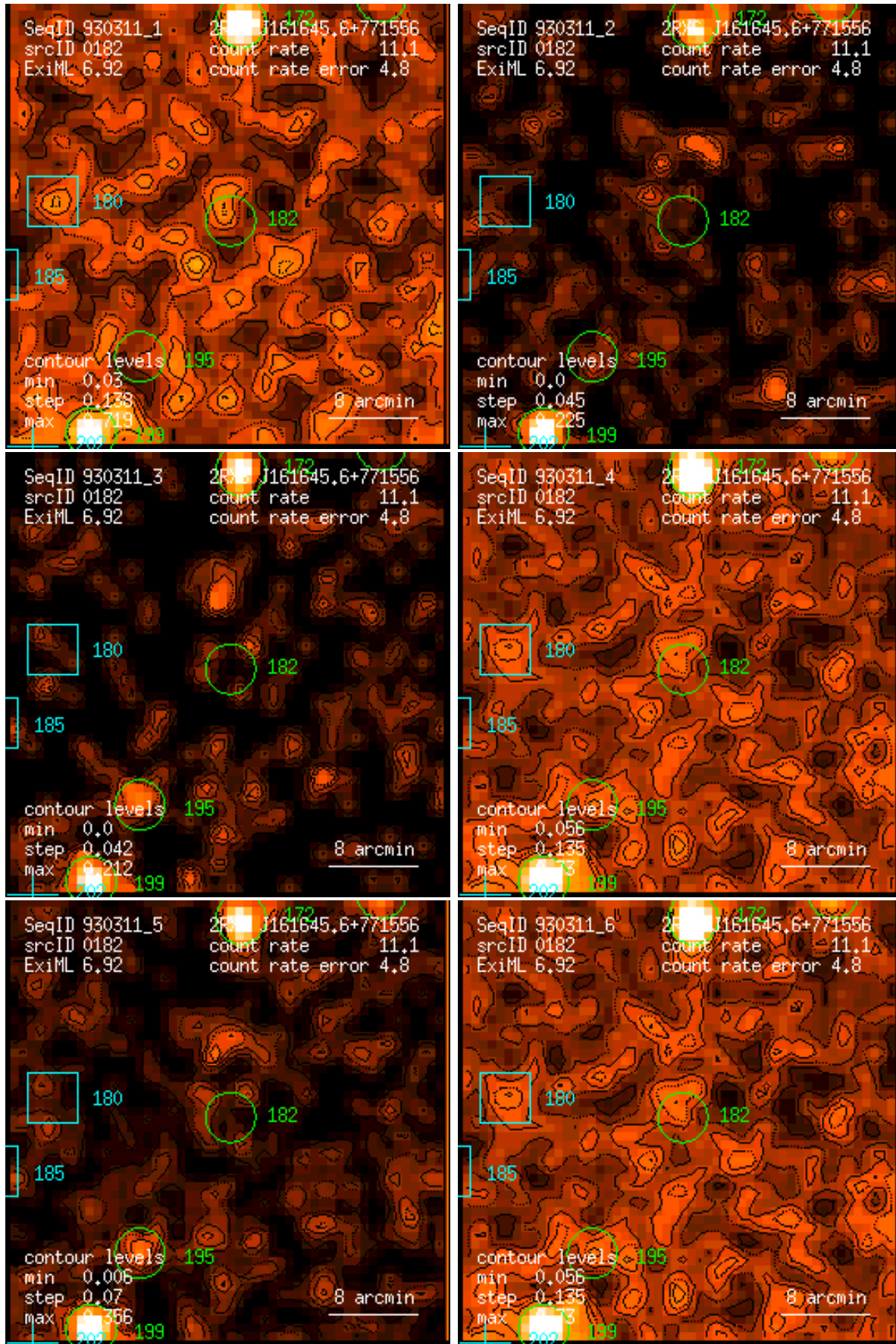
Figure 182: RASS 930311: detection 0182: band rate images, Gaussian filter: (1) PSPC channels 11 – 41, (2) 52 – 90, (3) 91 – 201, (4) 11 – 235, (5) 52 – 201, (6) 11 – 201. Broad band rates in counts/ks. Band rate contour levels in counts/ks/arcmin 2 .
