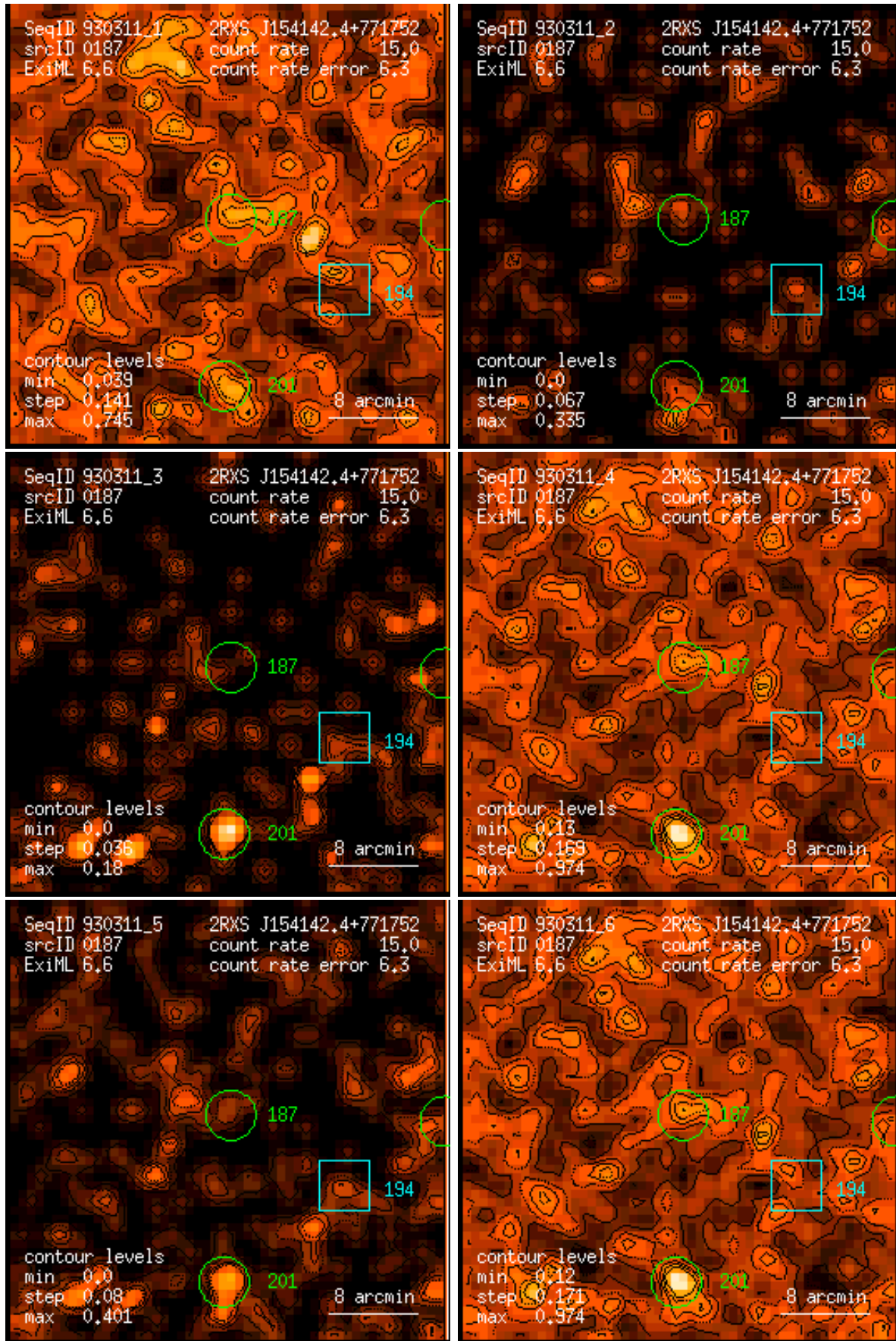
Figure 187: RASS 930311: detection 0187: band rate images, Gaussian filter: (1) PSPC channels 11 – 41, (2) 52 – 90, (3) 91 – 201, (4) 11 – 235, (5) 52 – 201, (6) 11 – 201. Broad band rates in counts/ks. Band rate contour levels in counts/ks/arcmin 2 .
