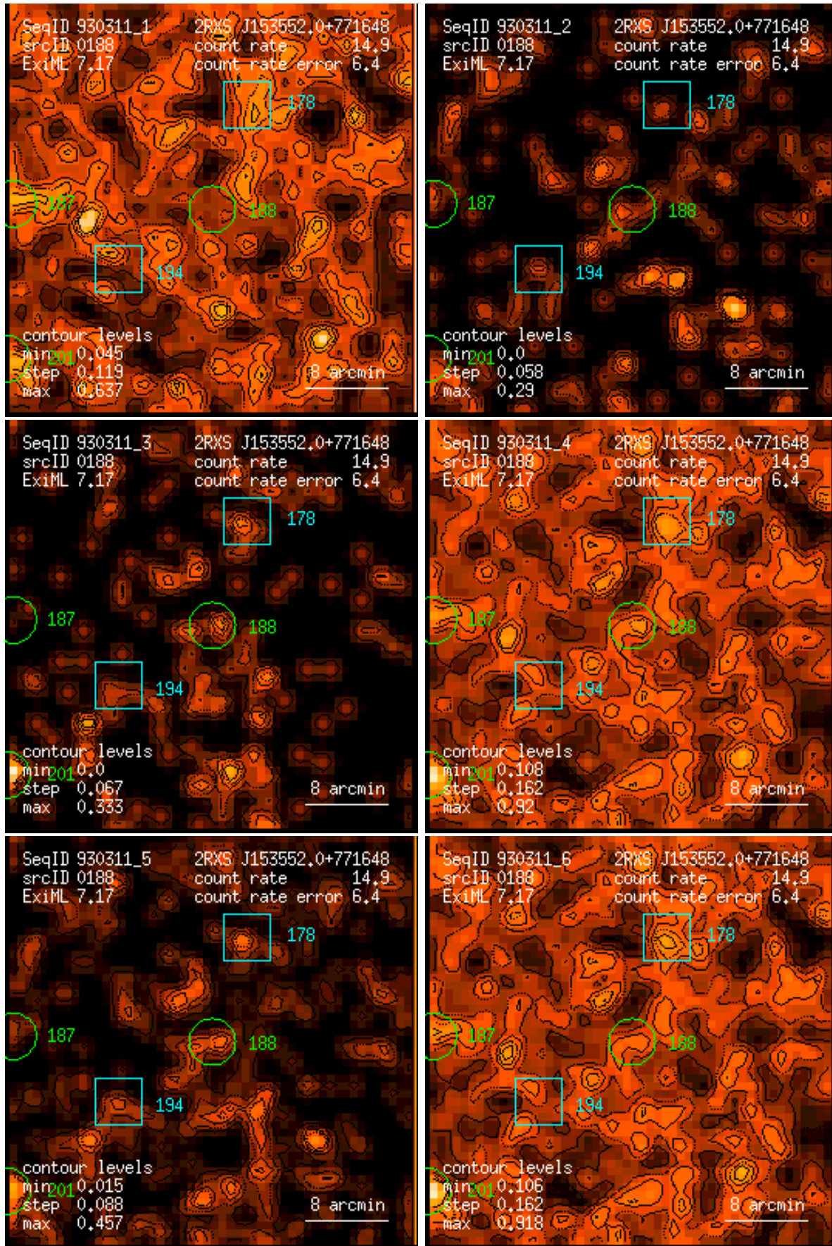
Figure 188: RASS 930311: detection 0188: band rate images, Gaussian filter: (1) PSPC channels 11 – 41, (2) 52 – 90, (3) 91 – 201, (4) 11 – 235, (5) 52 – 201, (6) 11 – 201. Broad band rates in counts/ks. Band rate contour levels in counts/ks/arcmin 2 .
