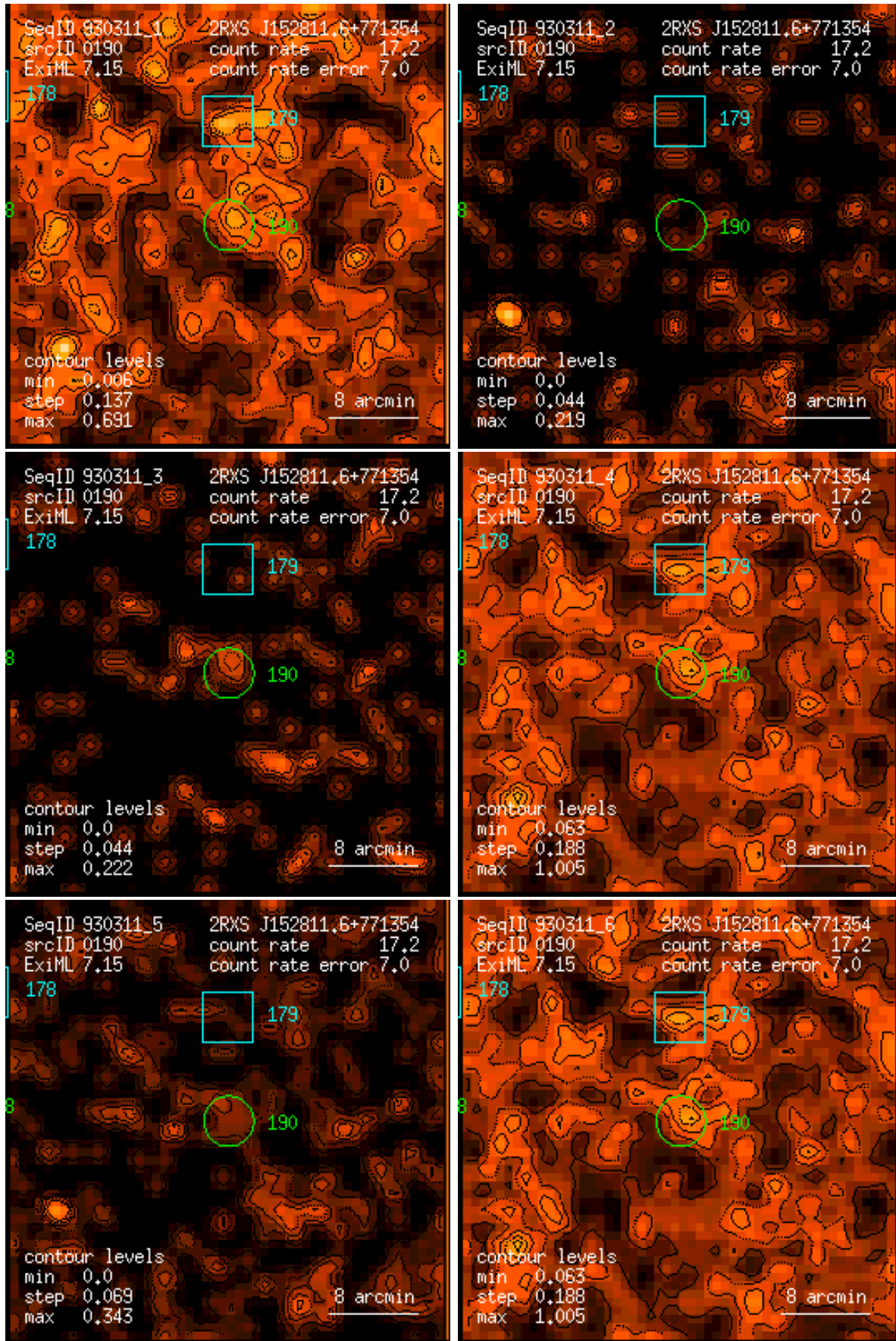
Figure 190: RASS 930311: detection 0190: band rate images, Gaussian filter: (1) PSPC channels 11 – 41, (2) 52 – 90, (3) 91 – 201, (4) 11 – 235, (5) 52 – 201, (6) 11 – 201. Broad band rates in counts/ks. Band rate contour levels in counts/ks/arcmin 2 .
