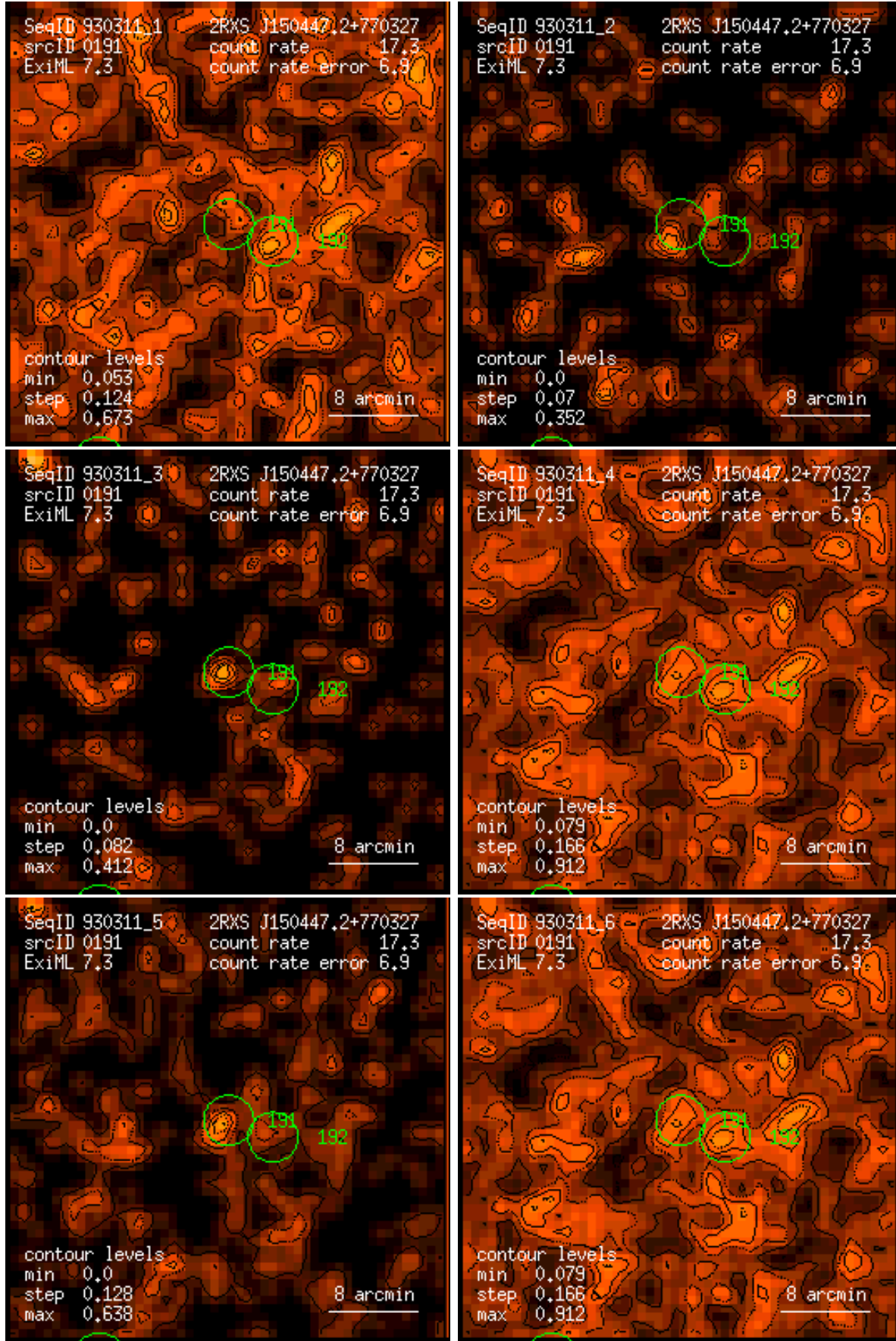
Figure 191: RASS 930311: detection 0191: band rate images, Gaussian filter: (1) PSPC channels 11 – 41, (2) 52 – 90, (3) 91 – 201, (4) 11 – 235, (5) 52 – 201, (6) 11 – 201. Broad band rates in counts/ks. Band rate contour levels in counts/ks/arcmin 2 .
