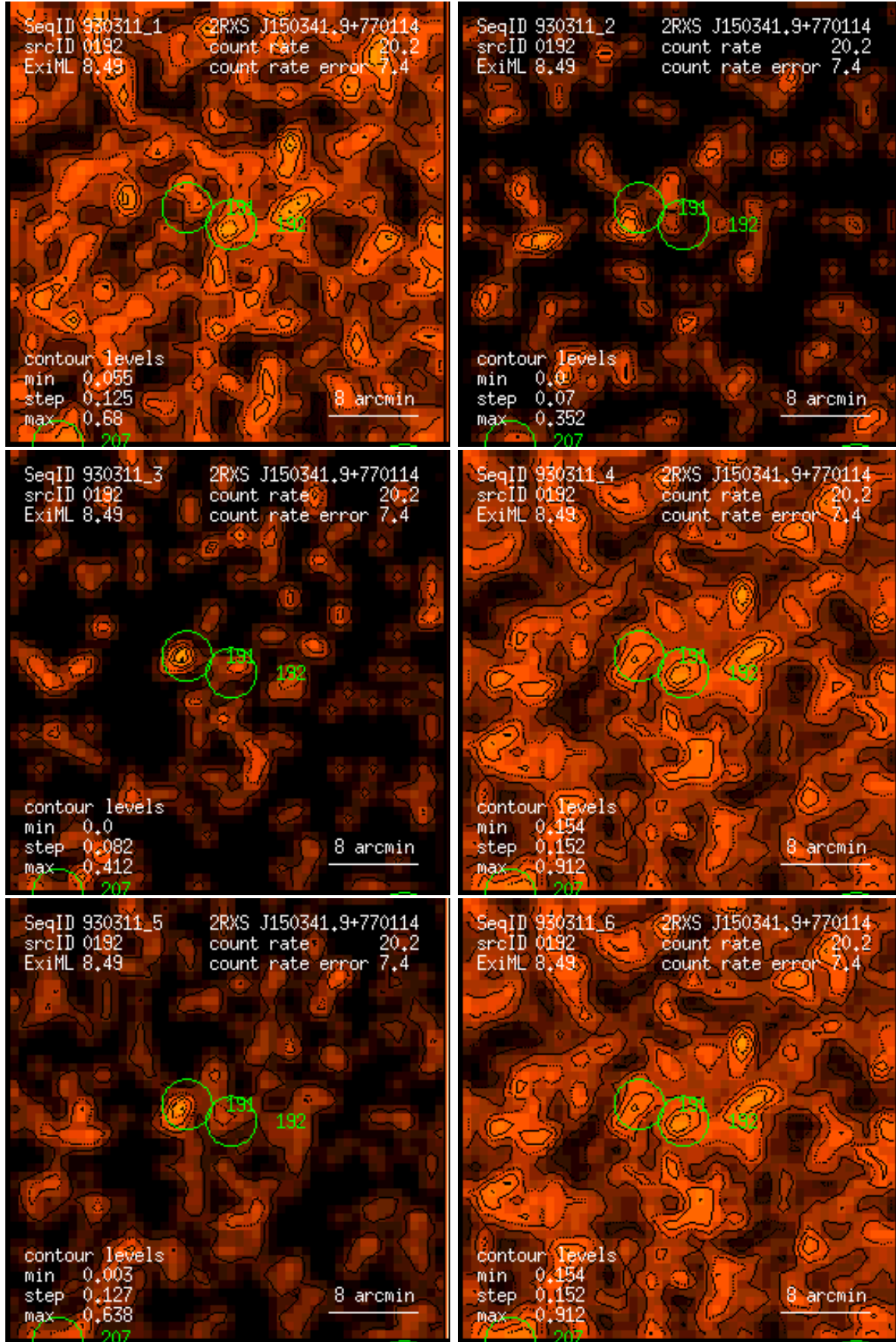
Figure 192: RASS 930311: detection 0192: band rate images, Gaussian filter: (1) PSPC channels 11 – 41, (2) 52 – 90, (3) 91 – 201, (4) 11 – 235, (5) 52 – 201, (6) 11 – 201. Broad band rates in counts/ks. Band rate contour levels in counts/ks/arcmin 2 .
