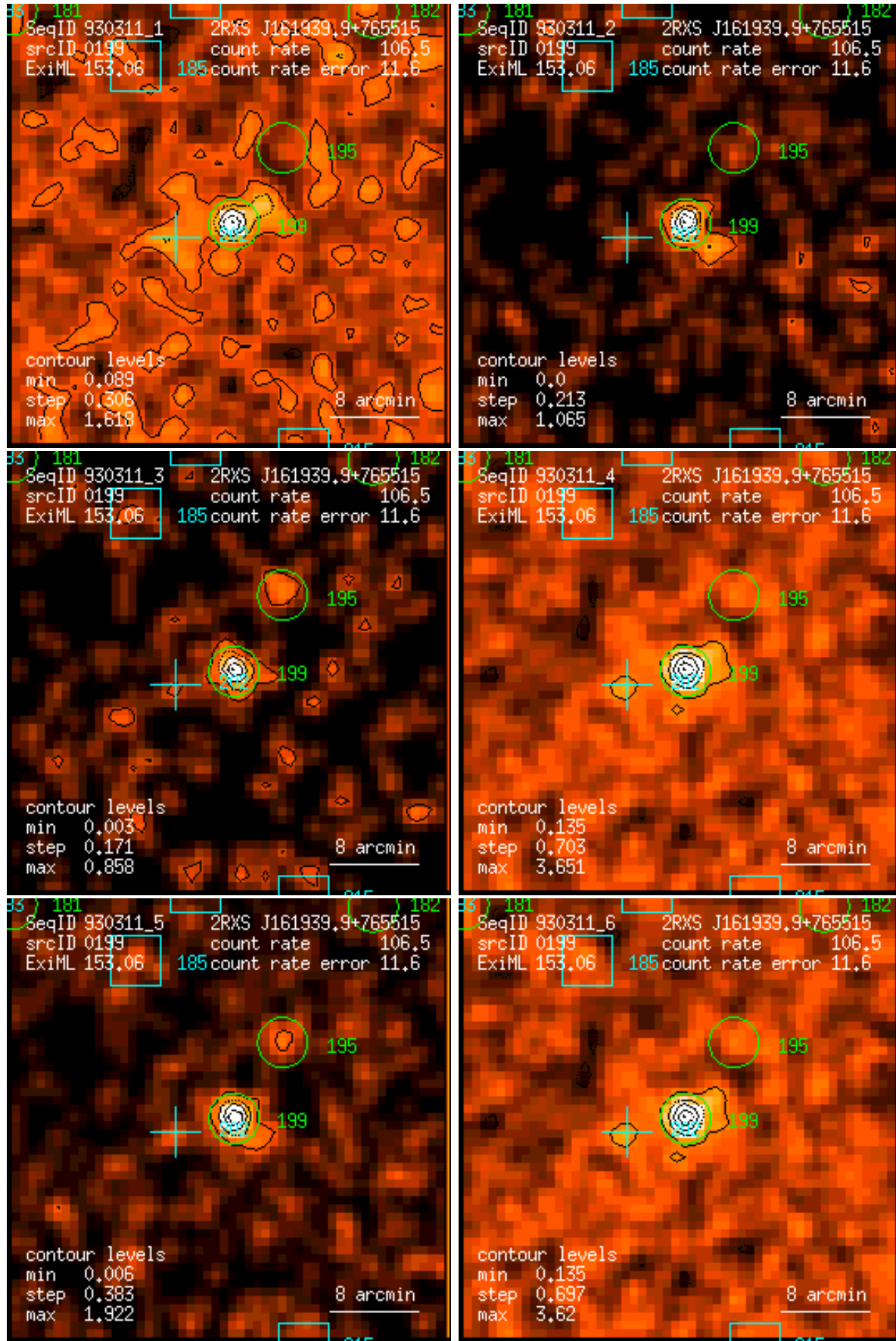
Figure 199: RASS 930311: detection 0199: band rate images, Gaussian filter: (1) PSPC channels 11 – 41, (2) 52 – 90, (3) 91 – 201, (4) 11 – 235, (5) 52 – 201, (6) 11 – 201. Broad band rates in counts/ks. Band rate contour levels in counts/ks/arcmin 2 .
