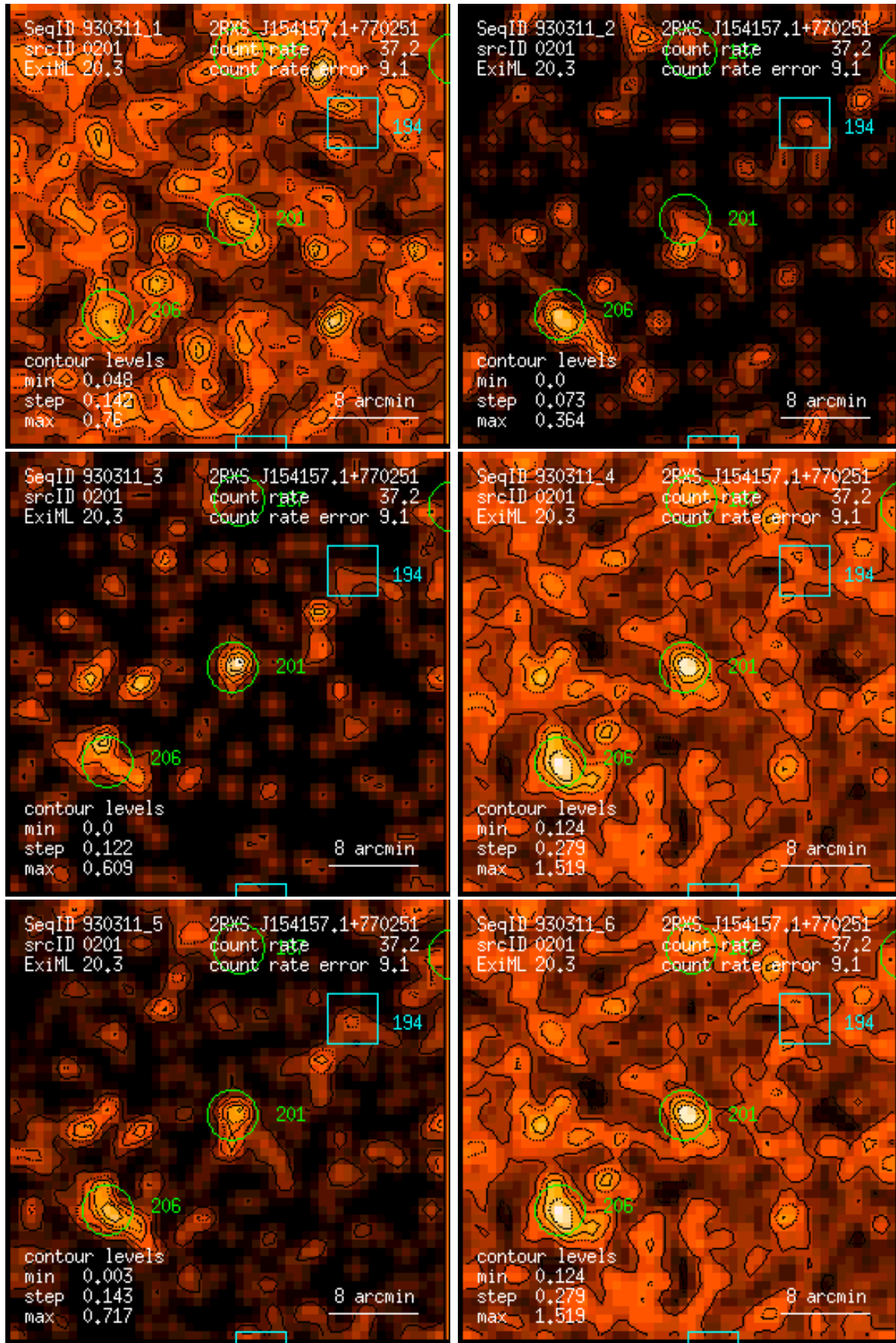
Figure 201: RASS 930311: detection 0201: band rate images, Gaussian filter: (1) PSPC channels 11 – 41, (2) 52 – 90, (3) 91 – 201, (4) 11 – 235, (5) 52 – 201, (6) 11 – 201. Broad band rates in counts/ks. Band rate contour levels in counts/ks/arcmin 2 .
