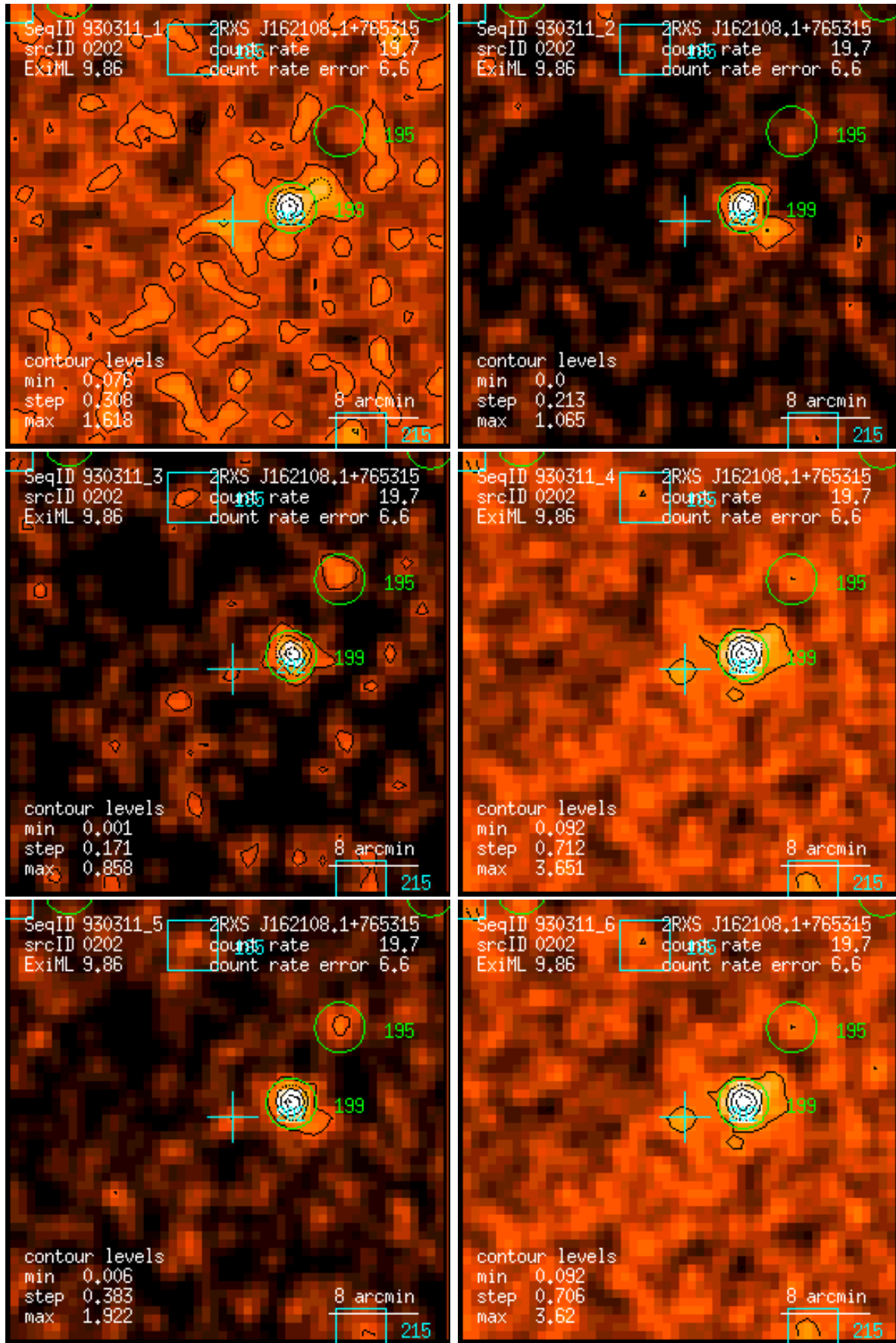
Figure 202: RASS 930311: detection 0202: band rate images, Gaussian filter: (1) PSPC channels 11 – 41, (2) 52 – 90, (3) 91 – 201, (4) 11 – 235, (5) 52 – 201, (6) 11 – 201. Broad band rates in counts/ks. Band rate contour levels in counts/ks/arcmin 2 .
