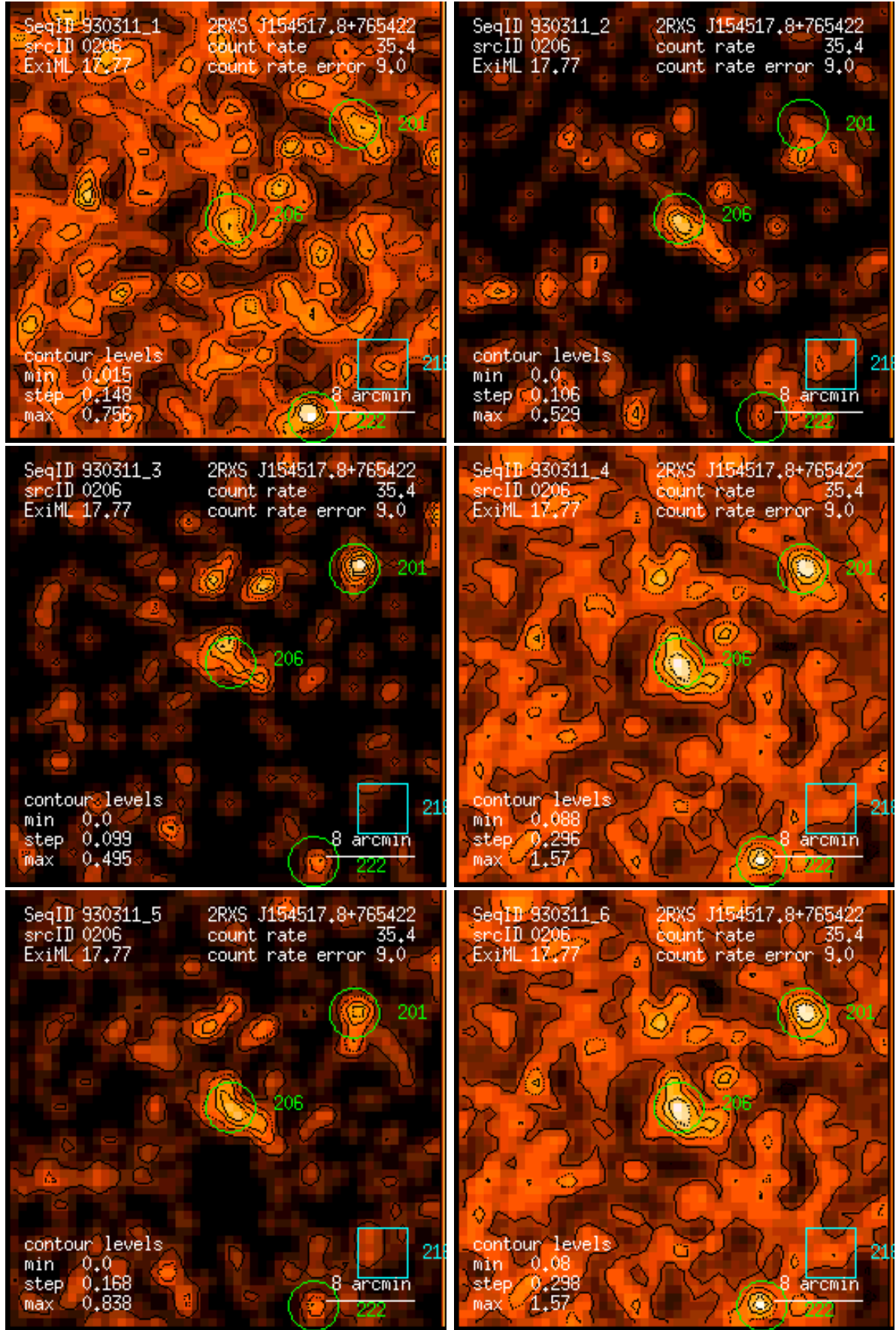
Figure 206: RASS 930311: detection 0206: band rate images, Gaussian filter: (1) PSPC channels 11 – 41, (2) 52 – 90, (3) 91 – 201, (4) 11 – 235, (5) 52 – 201, (6) 11 – 201. Broad band rates in counts/ks. Band rate contour levels in counts/ks/arcmin 2 .
