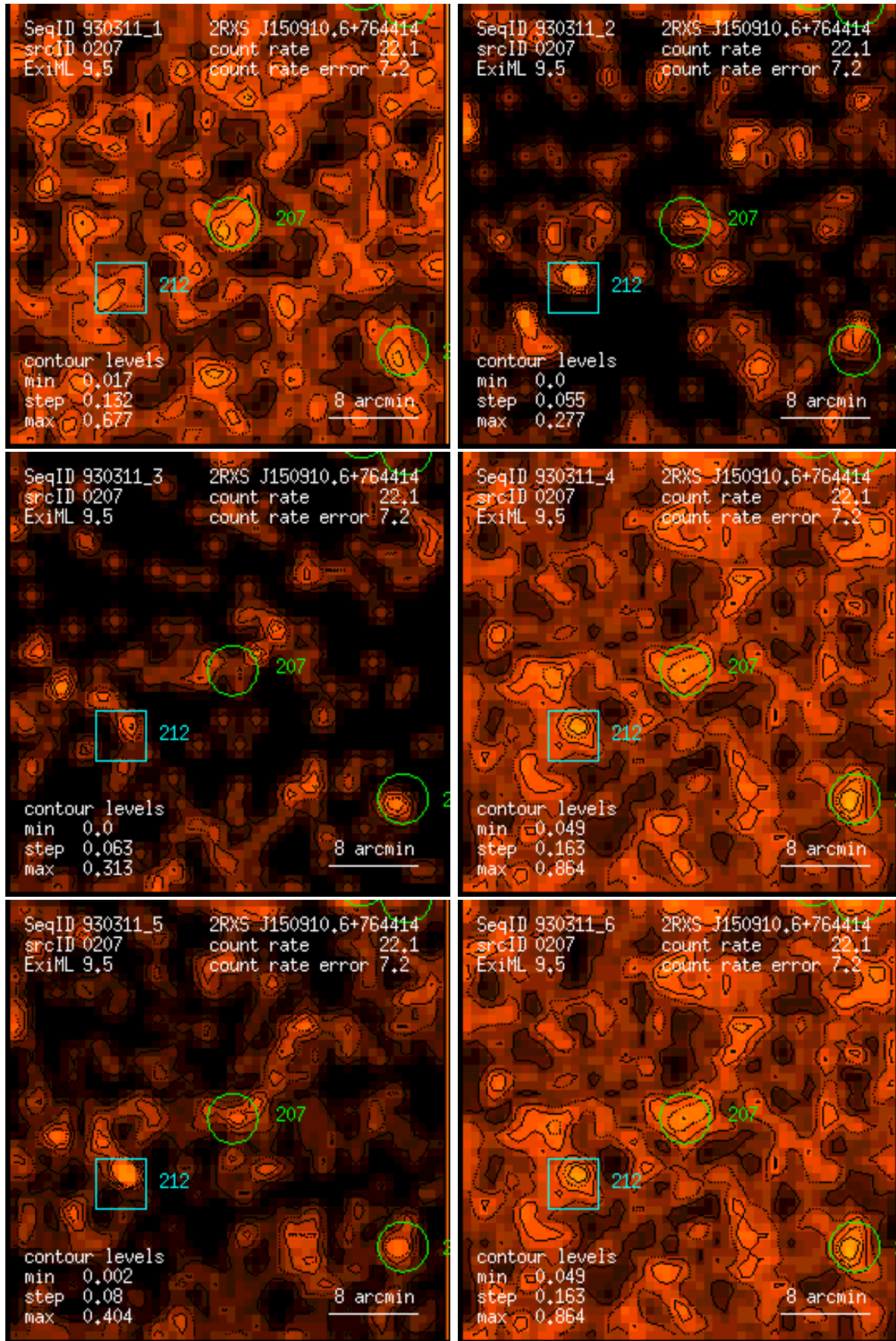
Figure 207: RASS 930311: detection 0207: band rate images, Gaussian filter: (1) PSPC channels 11 – 41, (2) 52 – 90, (3) 91 – 201, (4) 11 – 235, (5) 52 – 201, (6) 11 – 201. Broad band rates in counts/ks. Band rate contour levels in counts/ks/arcmin 2 .
