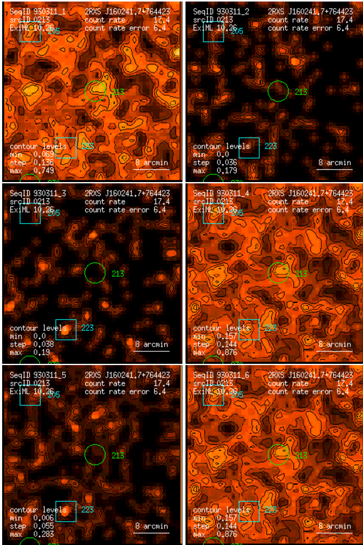
Figure 213: RASS 930311: detection 0213: band rate images, Gaussian filter: (1) PSPC channels 11 – 41, (2) 52 – 90, (3) 91 – 201, (4) 11 – 235, (5) 52 – 201, (6) 11 – 201. Broad band rates in counts/ks. Band rate contour levels in counts/ks/arcmin 2 .
