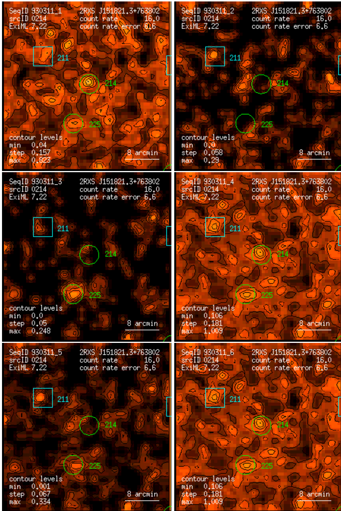
Figure 214: RASS 930311: detection 0214: band rate images, Gaussian filter: (1) PSPC channels 11 – 41, (2) 52 – 90, (3) 91 – 201, (4) 11 – 235, (5) 52 – 201, (6) 11 – 201. Broad band rates in counts/ks. Band rate contour levels in counts/ks/arcmin 2 .
