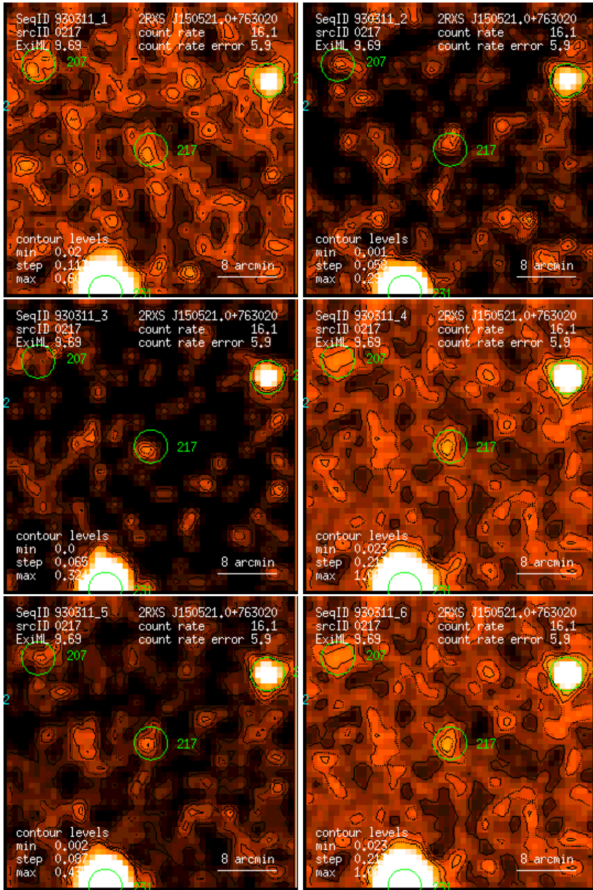
Figure 217: RASS 930311: detection 0217: band rate images, Gaussian filter: (1) PSPC channels 11 – 41, (2) 52 – 90, (3) 91 – 201, (4) 11 – 235, (5) 52 – 201, (6) 11 – 201. Broad band rates in counts/ks. Band rate contour levels in counts/ks/arcmin 2 .
