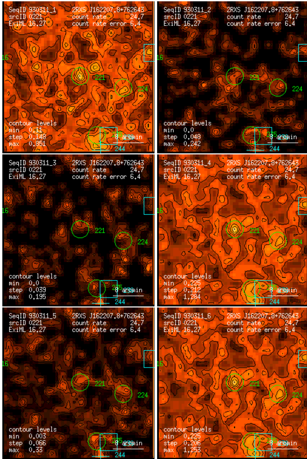
Figure 221: RASS 930311: detection 0221: band rate images, Gaussian filter: (1) PSPC channels 11 – 41, (2) 52 – 90, (3) 91 – 201, (4) 11 – 235, (5) 52 – 201, (6) 11 – 201. Broad band rates in counts/ks. Band rate contour levels in counts/ks/arcmin 2 .
