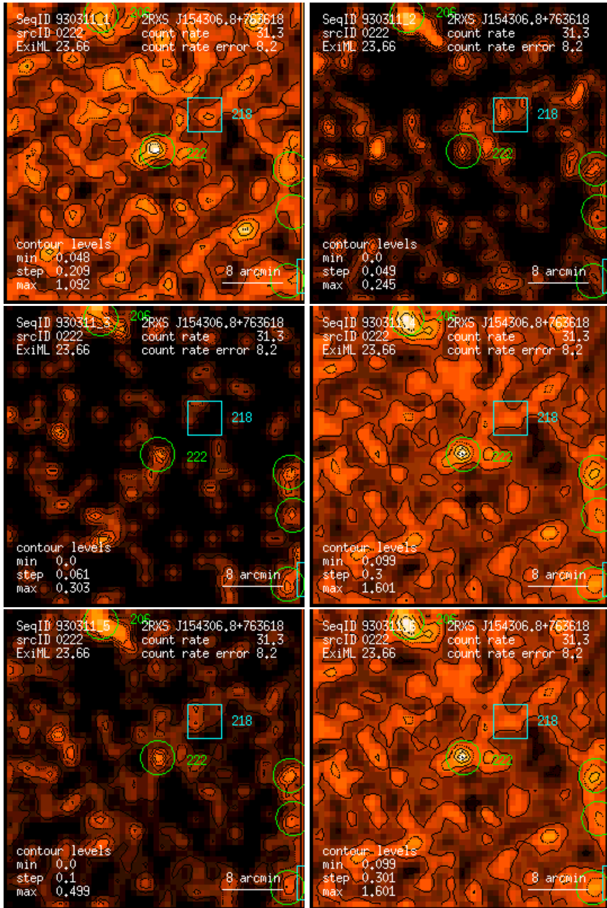
Figure 222: RASS 930311: detection 0222: band rate images, Gaussian filter: (1) PSPC channels 11 – 41, (2) 52 – 90, (3) 91 – 201, (4) 11 – 235, (5) 52 – 201, (6) 11 – 201. Broad band rates in counts/ks. Band rate contour levels in counts/ks/arcmin 2 .
