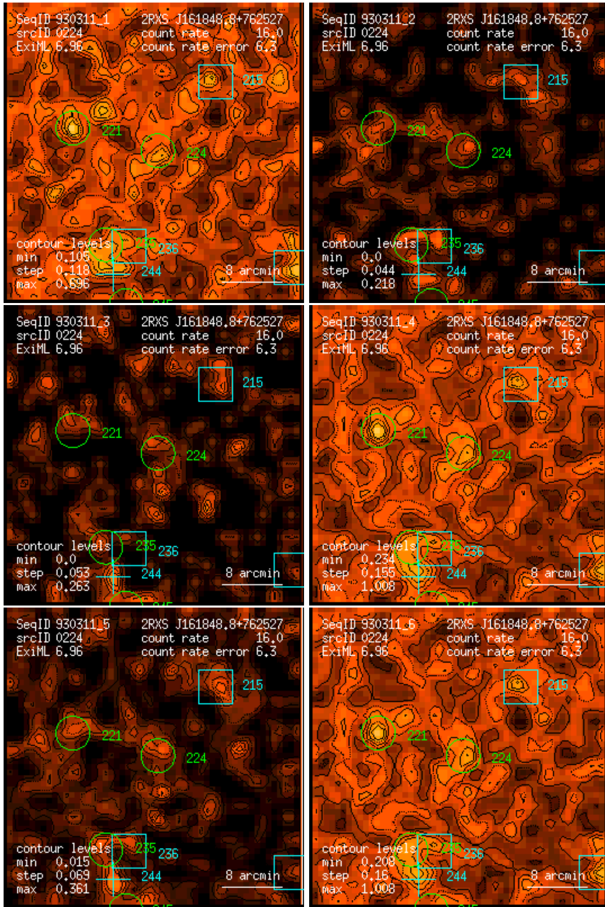
Figure 224: RASS 930311: detection 0224: band rate images, Gaussian filter: (1) PSPC channels 11 – 41, (2) 52 – 90, (3) 91 – 201, (4) 11 – 235, (5) 52 – 201, (6) 11 – 201. Broad band rates in counts/ks. Band rate contour levels in counts/ks/arcmin 2 .
