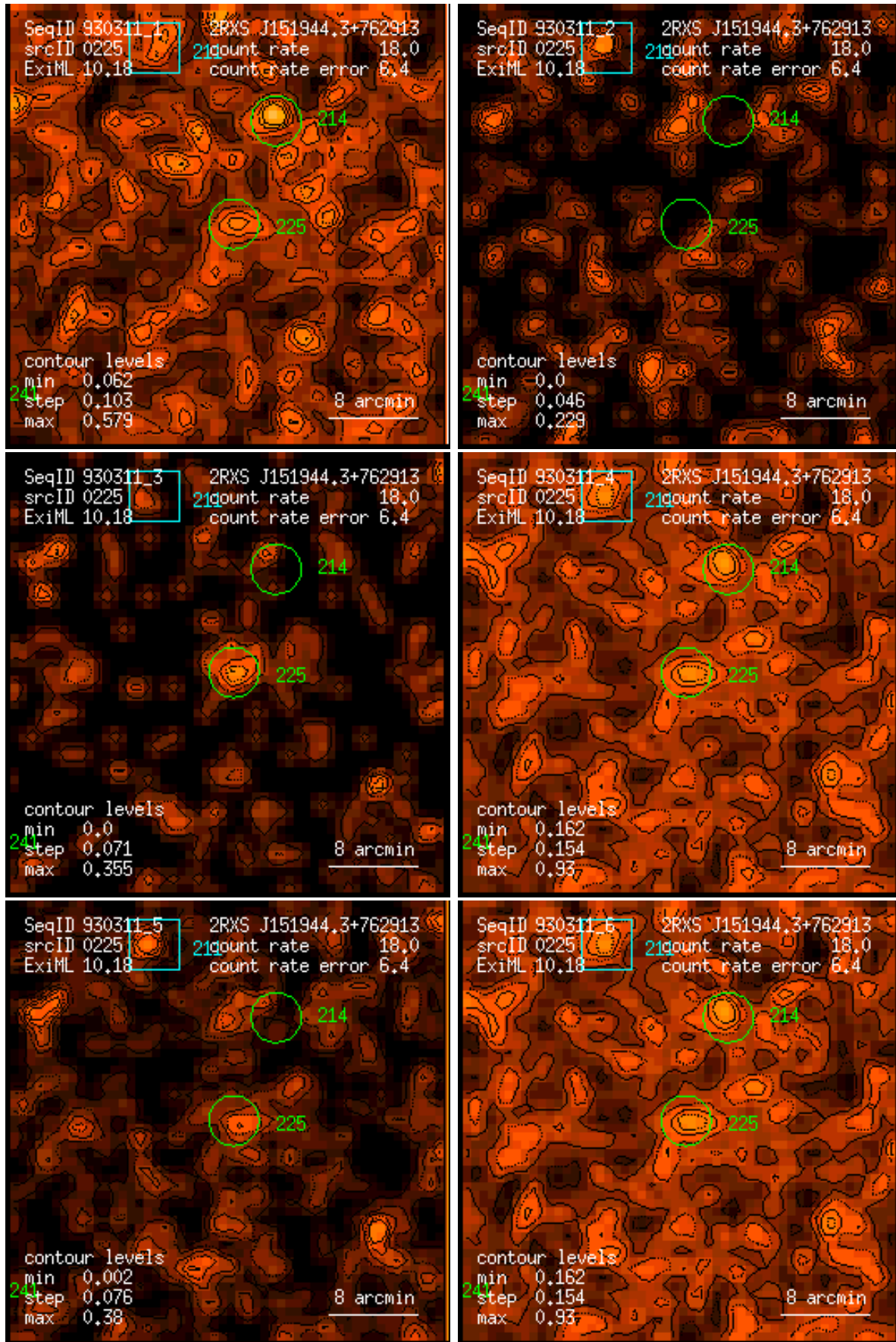
Figure 225: RASS 930311: detection 0225: band rate images, Gaussian filter: (1) PSPC channels 11 – 41, (2) 52 – 90, (3) 91 – 201, (4) 11 – 235, (5) 52 – 201, (6) 11 – 201. Broad band rates in counts/ks. Band rate contour levels in counts/ks/arcmin 2 .
