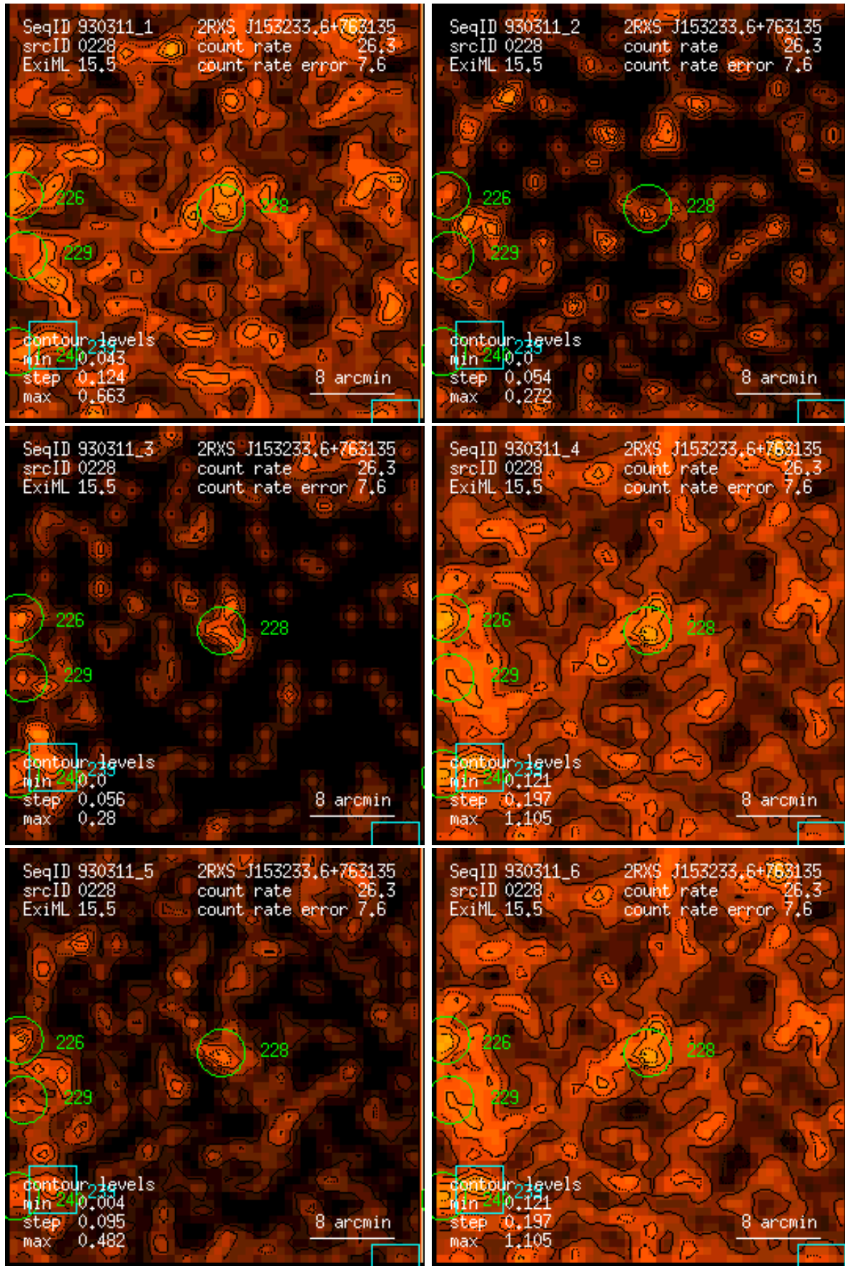
Figure 228: RASS 930311: detection 0228: band rate images, Gaussian filter: (1) PSPC channels 11 – 41, (2) 52 – 90, (3) 91 – 201, (4) 11 – 235, (5) 52 – 201, (6) 11 – 201. Broad band rates in counts/ks. Band rate contour levels in counts/ks/arcmin 2 .
