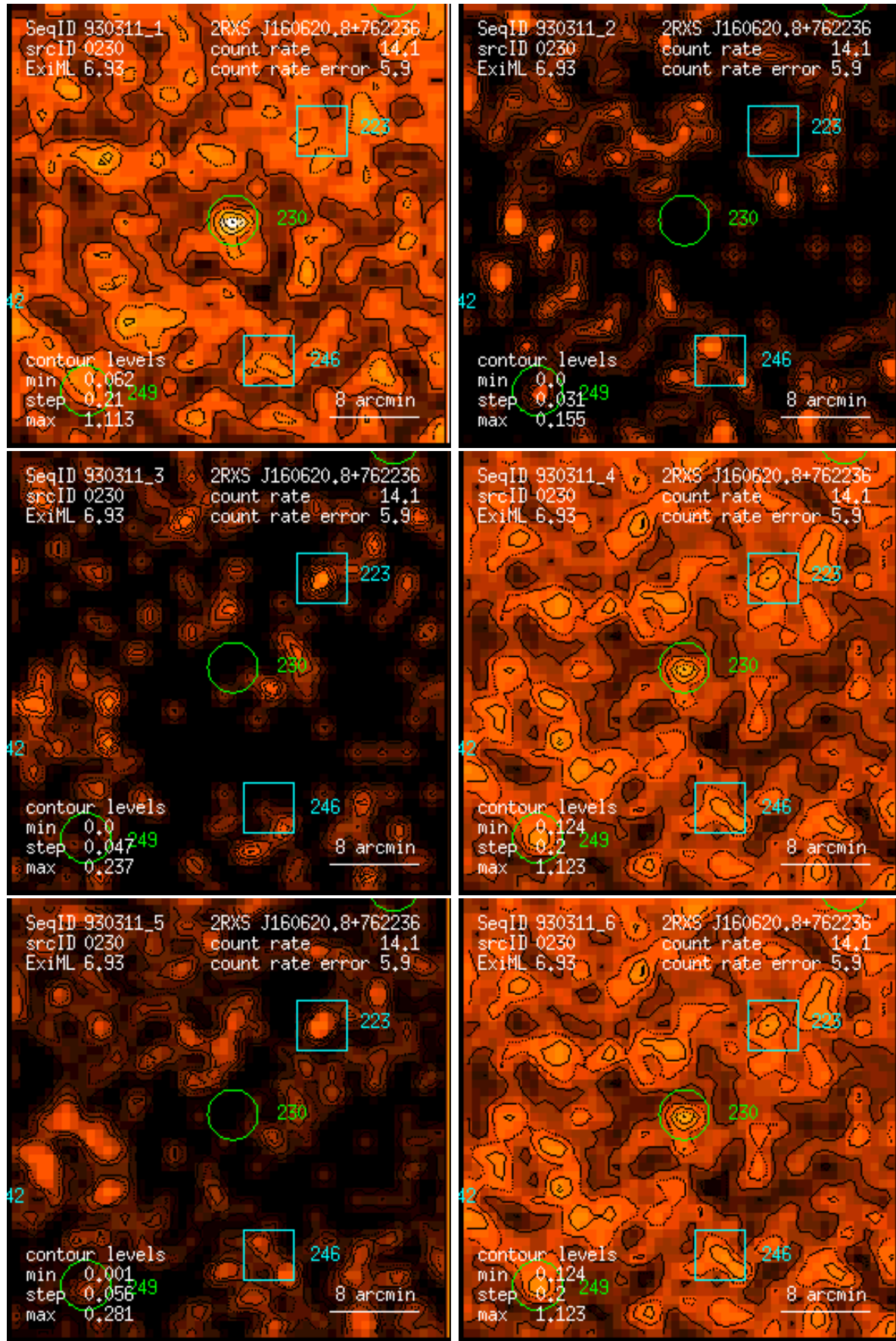
Figure 230: RASS 930311: detection 0230: band rate images, Gaussian filter: (1) PSPC channels 11 – 41, (2) 52 – 90, (3) 91 – 201, (4) 11 – 235, (5) 52 – 201, (6) 11 – 201. Broad band rates in counts/ks. Band rate contour levels in counts/ks/arcmin 2 .
