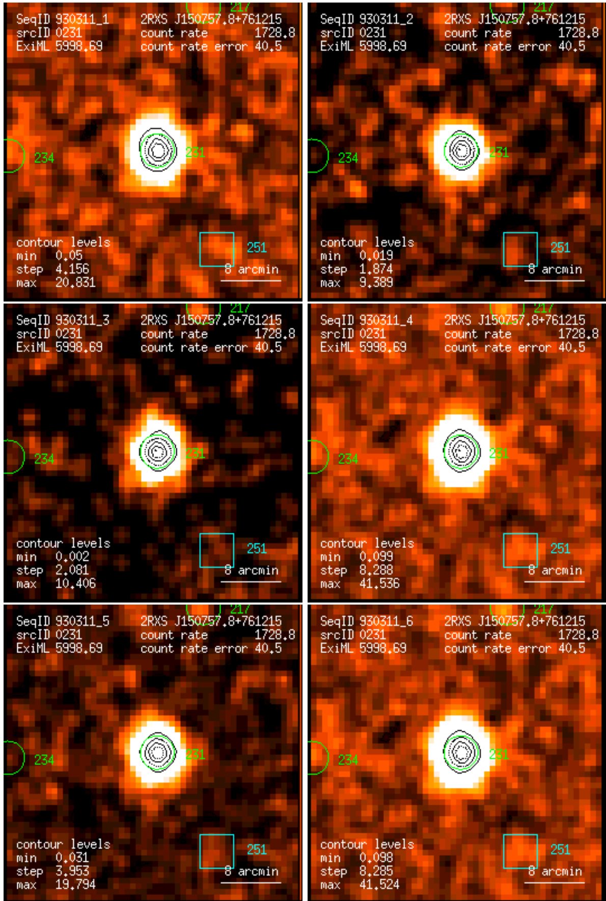
Figure 231: RASS 930311: detection 0231: band rate images, Gaussian filter: (1) PSPC channels 11 – 41, (2) 52 – 90, (3) 91 – 201, (4) 11 – 235, (5) 52 – 201, (6) 11 – 201. Broad band rates in counts/ks. Band rate contour levels in counts/ks/arcmin 2 .
