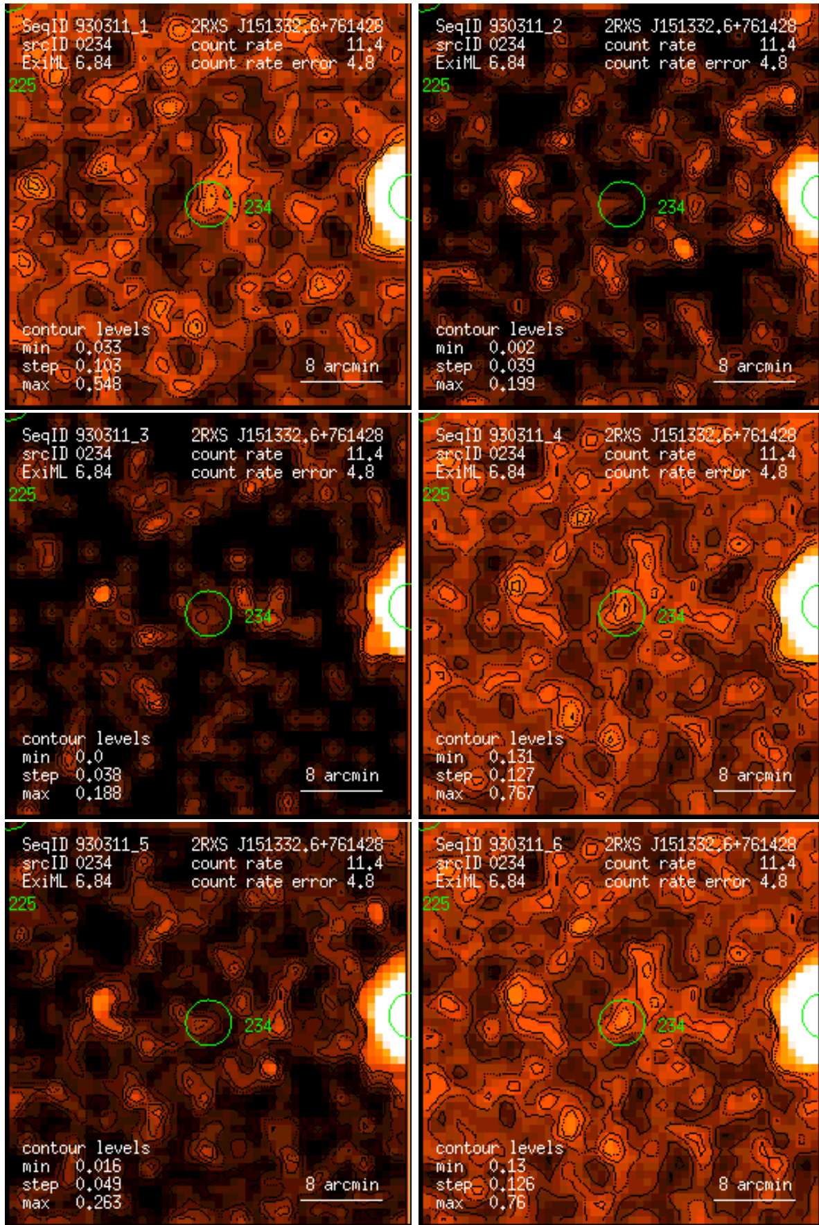
Figure 234: RASS 930311: detection 0234: band rate images, Gaussian filter: (1) PSPC channels 11 – 41, (2) 52 – 90, (3) 91 – 201, (4) 11 – 235, (5) 52 – 201, (6) 11 – 201. Broad band rates in counts/ks. Band rate contour levels in counts/ks/arcmin 2 .
