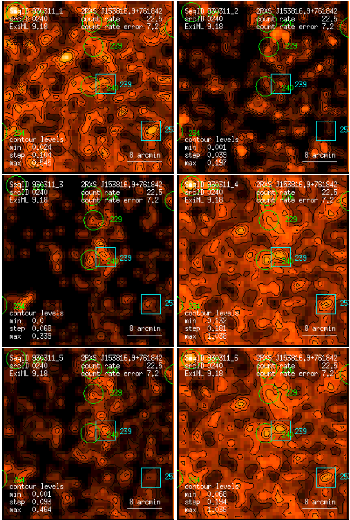
Figure 240: RASS 930311: detection 0240: band rate images, Gaussian filter: (1) PSPC channels 11 – 41, (2) 52 – 90, (3) 91 – 201, (4) 11 – 235, (5) 52 – 201, (6) 11 – 201. Broad band rates in counts/ks. Band rate contour levels in counts/ks/arcmin 2 .
