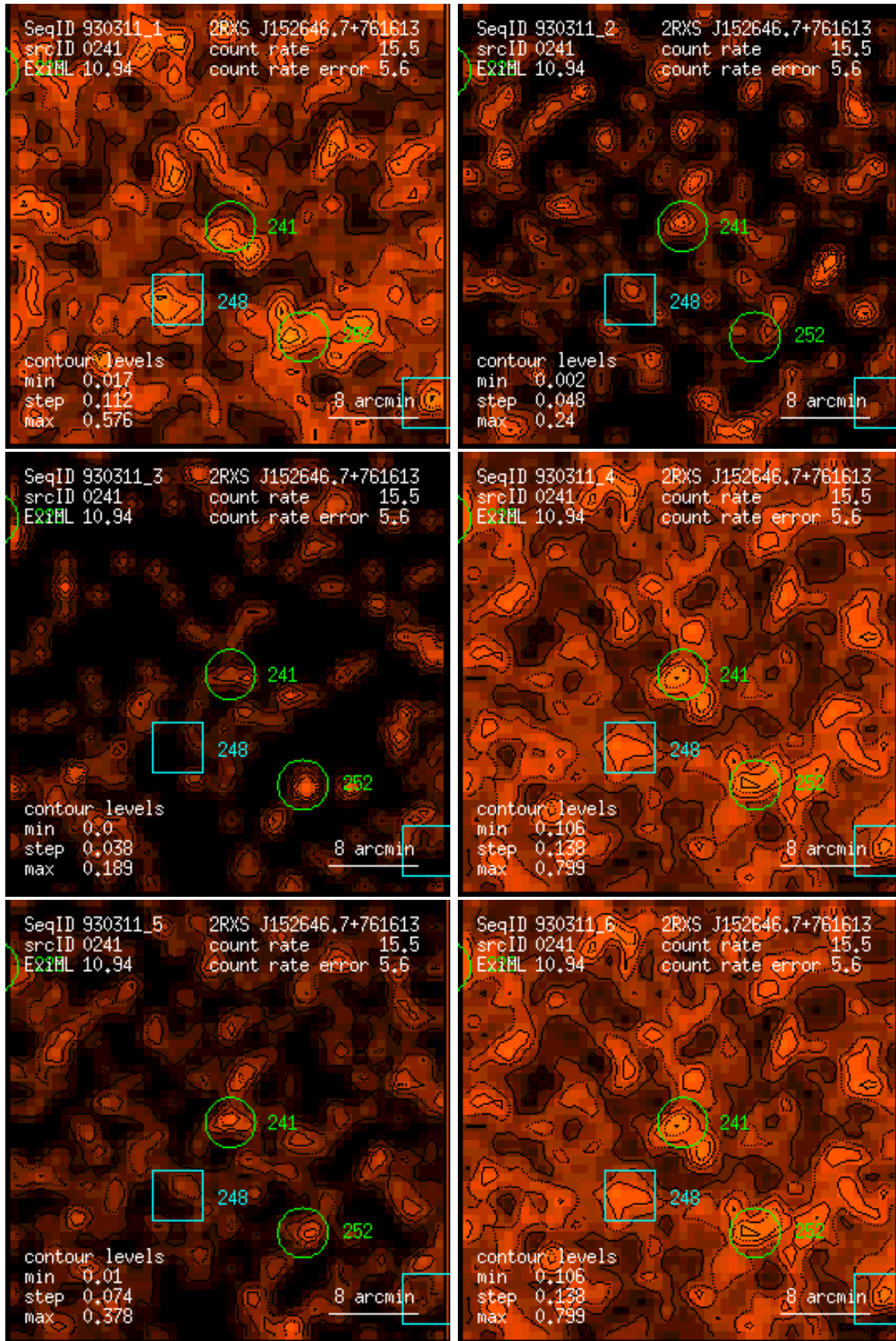
Figure 241: RASS 930311: detection 0241: band rate images, Gaussian filter: (1) PSPC channels 11 – 41, (2) 52 – 90, (3) 91 – 201, (4) 11 – 235, (5) 52 – 201, (6) 11 – 201. Broad band rates in counts/ks. Band rate contour levels in counts/ks/arcmin 2 .
