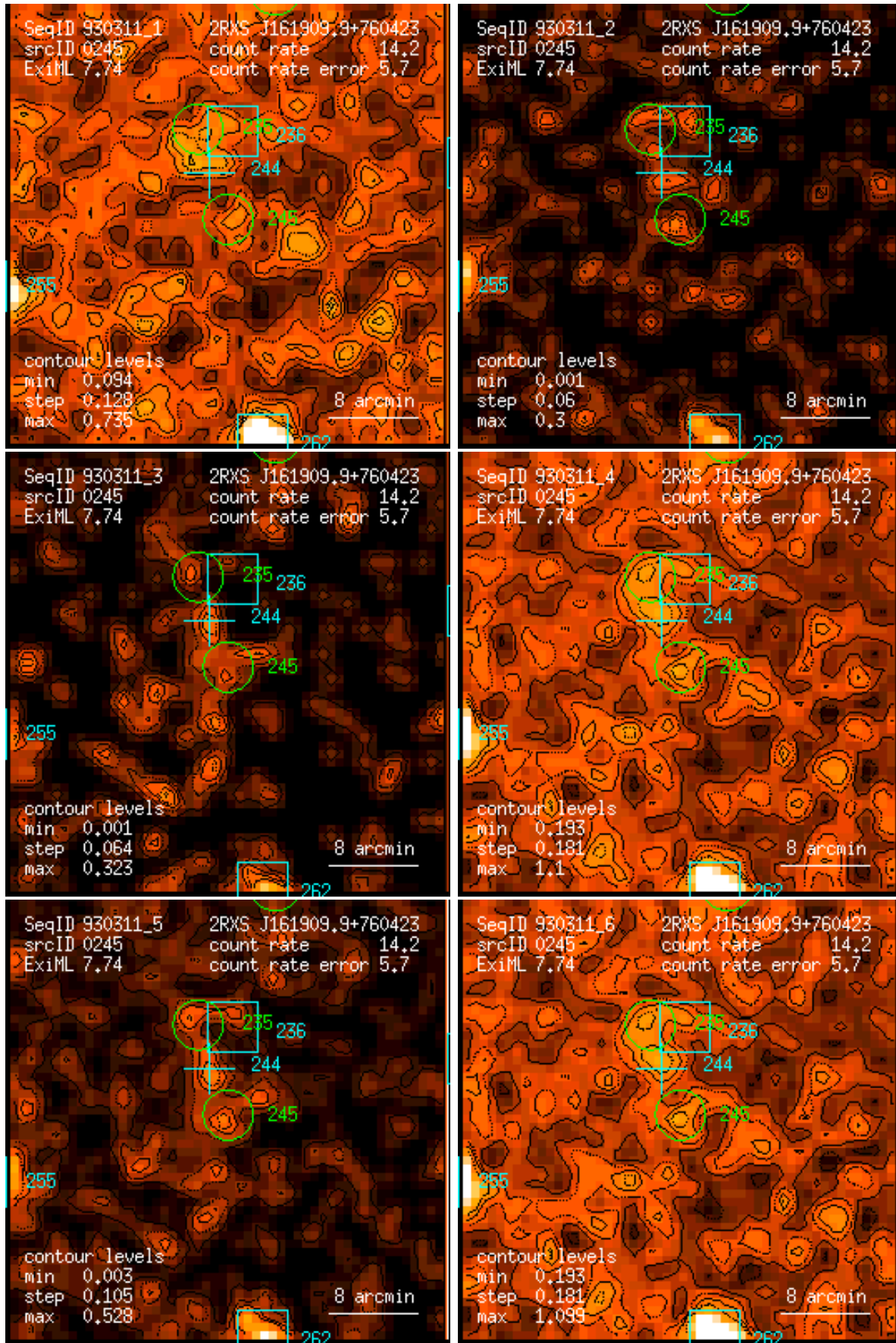
Figure 245: RASS 930311: detection 0245: band rate images, Gaussian filter: (1) PSPC channels 11 – 41, (2) 52 – 90, (3) 91 – 201, (4) 11 – 235, (5) 52 – 201, (6) 11 – 201. Broad band rates in counts/ks. Band rate contour levels in counts/ks/arcmin 2 .
