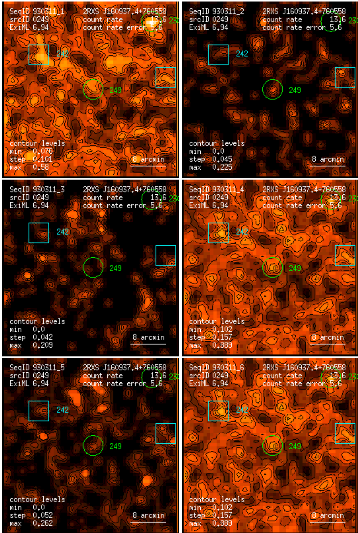
Figure 249: RASS 930311: detection 0249: band rate images, Gaussian filter: (1) PSPC channels 11 – 41, (2) 52 – 90, (3) 91 – 201, (4) 11 – 235, (5) 52 – 201, (6) 11 – 201. Broad band rates in counts/ks. Band rate contour levels in counts/ks/arcmin 2 .
