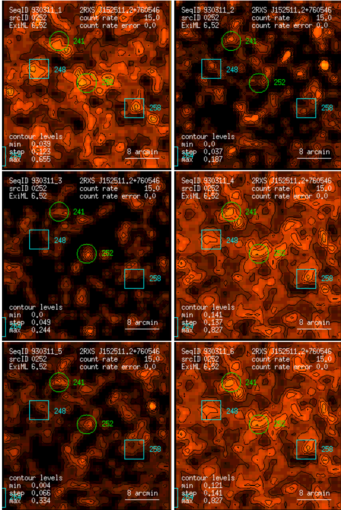
Figure 252: RASS 930311: detection 0252: band rate images, Gaussian filter: (1) PSPC channels 11 – 41, (2) 52 – 90, (3) 91 – 201, (4) 11 – 235, (5) 52 – 201, (6) 11 – 201. Broad band rates in counts/ks. Band rate contour levels in counts/ks/arcmin 2 .
