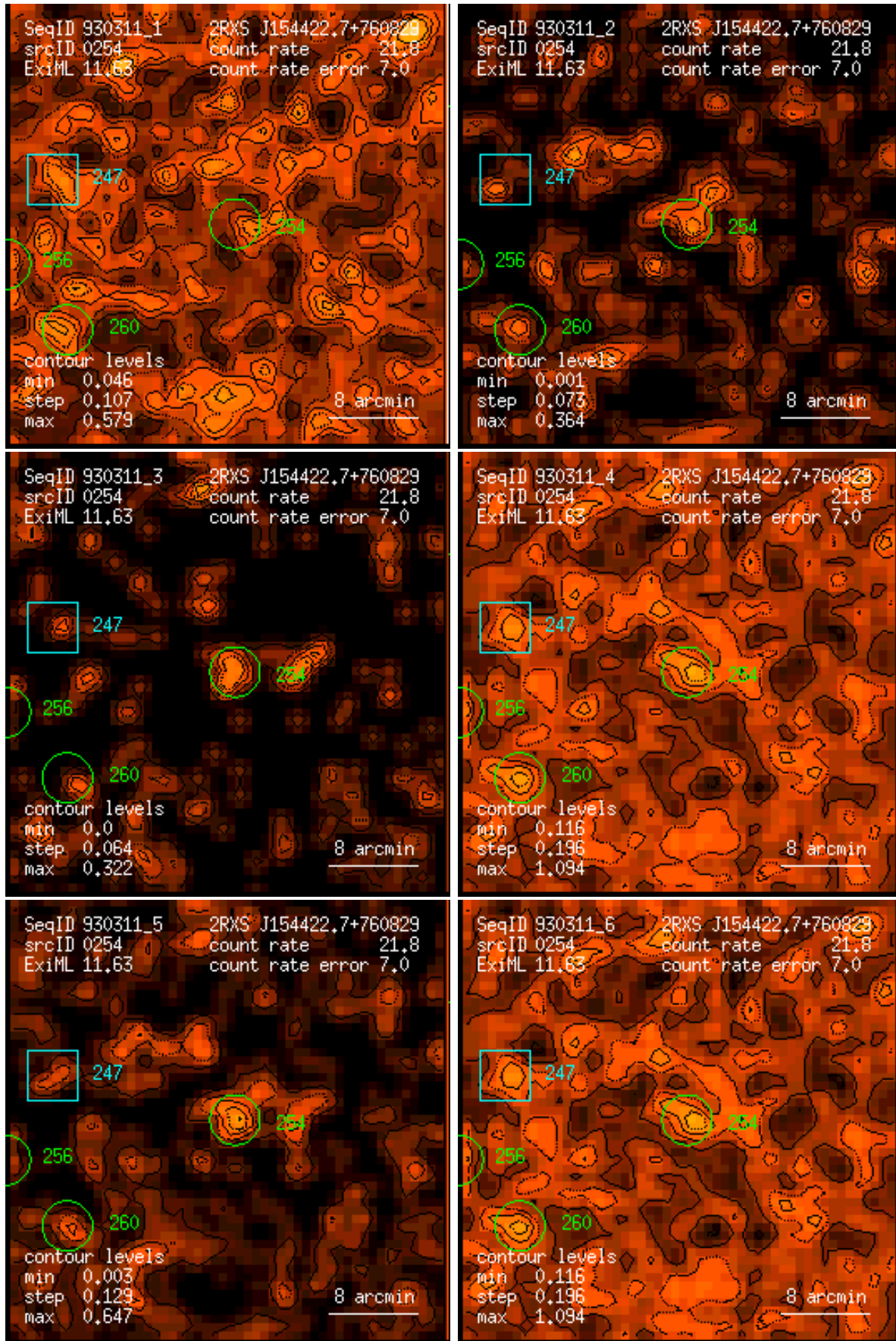
Figure 254: RASS 930311: detection 0254: band rate images, Gaussian filter: (1) PSPC channels 11 – 41, (2) 52 – 90, (3) 91 – 201, (4) 11 – 235, (5) 52 – 201, (6) 11 – 201. Broad band rates in counts/ks. Band rate contour levels in counts/ks/arcmin 2 .
