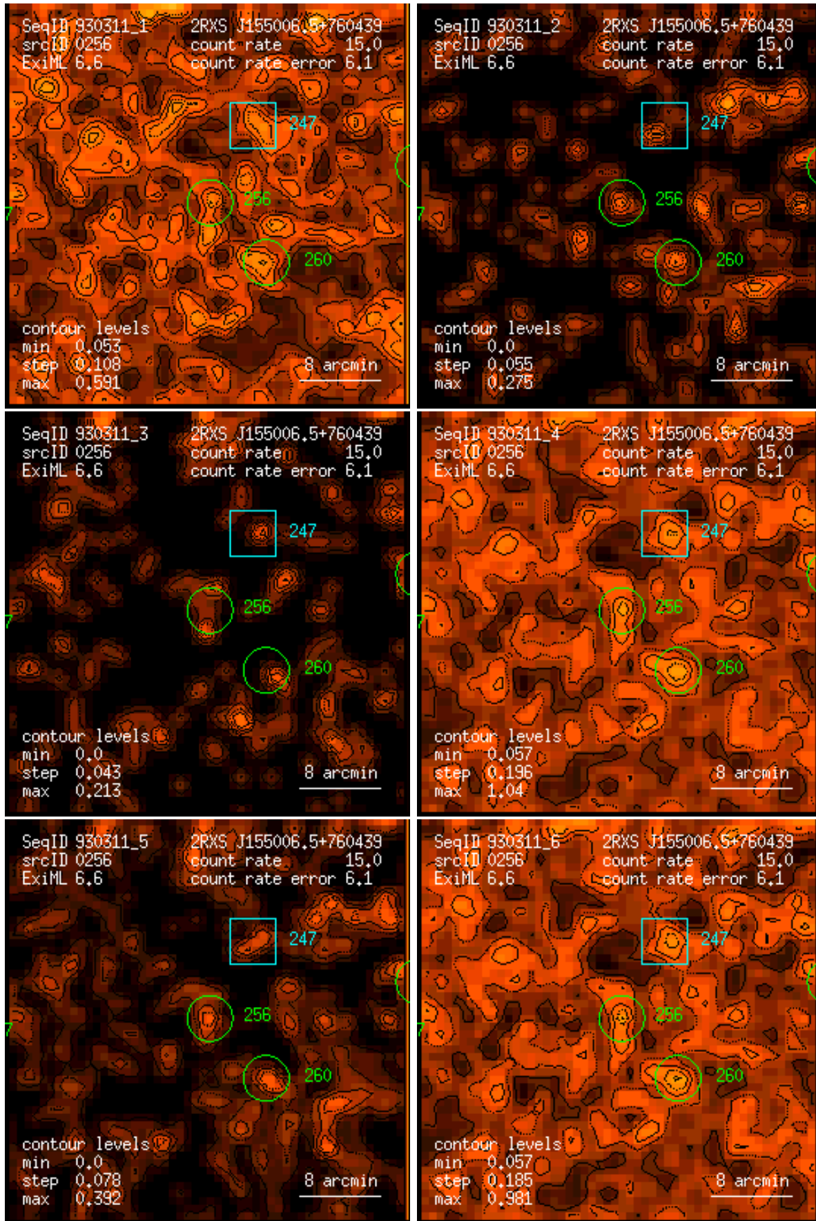
Figure 256: RASS 930311: detection 0256: band rate images, Gaussian filter: (1) PSPC channels 11 – 41, (2) 52 – 90, (3) 91 – 201, (4) 11 – 235, (5) 52 – 201, (6) 11 – 201. Broad band rates in counts/ks. Band rate contour levels in counts/ks/arcmin 2 .
