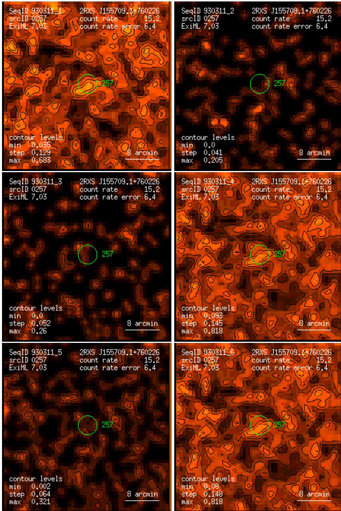
Figure 257: RASS 930311: detection 0257: band rate images, Gaussian filter: (1) PSPC channels 11 – 41, (2) 52 – 90, (3) 91 – 201, (4) 11 – 235, (5) 52 – 201, (6) 11 – 201. Broad band rates in counts/ks. Band rate contour levels in counts/ks/arcmin 2 .
