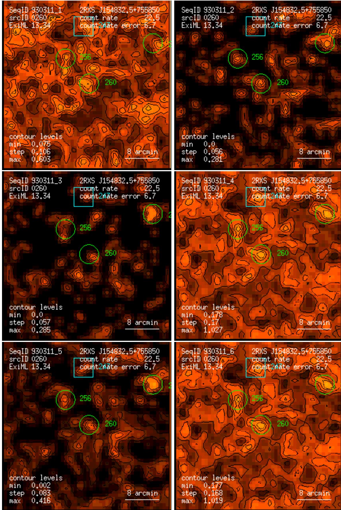
Figure 260: RASS 930311: detection 0260: band rate images, Gaussian filter: (1) PSPC channels 11 – 41, (2) 52 – 90, (3) 91 – 201, (4) 11 – 235, (5) 52 – 201, (6) 11 – 201. Broad band rates in counts/ks. Band rate contour levels in counts/ks/arcmin 2 .
