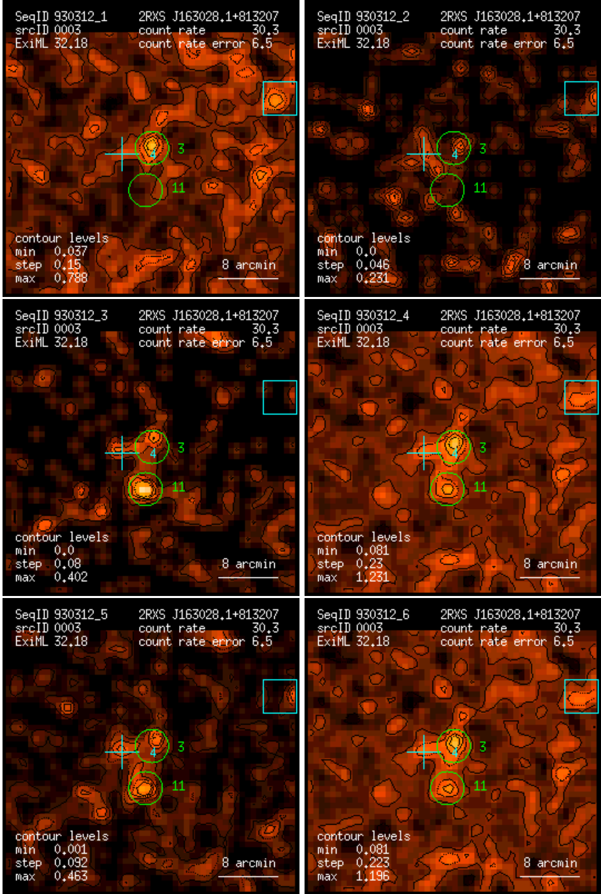
Figure 3: RASS 930312: detection 0003: band rate images, Gaussian filter: (1) PSPC channels 11 – 41, (2) 52 – 90, (3) 91 – 201, (4) 11 – 235, (5) 52 – 201, (6) 11 – 201. Broad band rates in counts/ks. Band rate contour levels in counts/ks/arcmin 2 .
