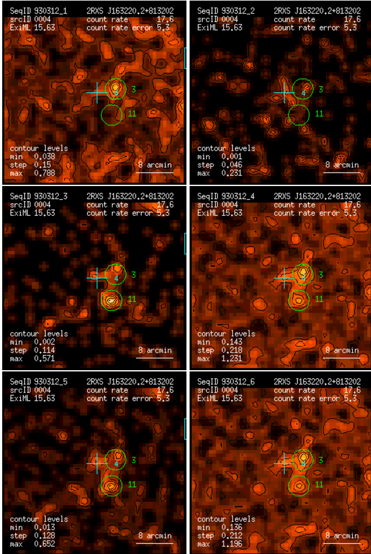
Figure 4: RASS 930312: detection 0004: band rate images, Gaussian filter: (1) PSPC channels 11 – 41, (2) 52 – 90, (3) 91 – 201, (4) 11 – 235, (5) 52 – 201, (6) 11 – 201. Broad band rates in counts/ks. Band rate contour levels in counts/ks/arcmin 2 .
