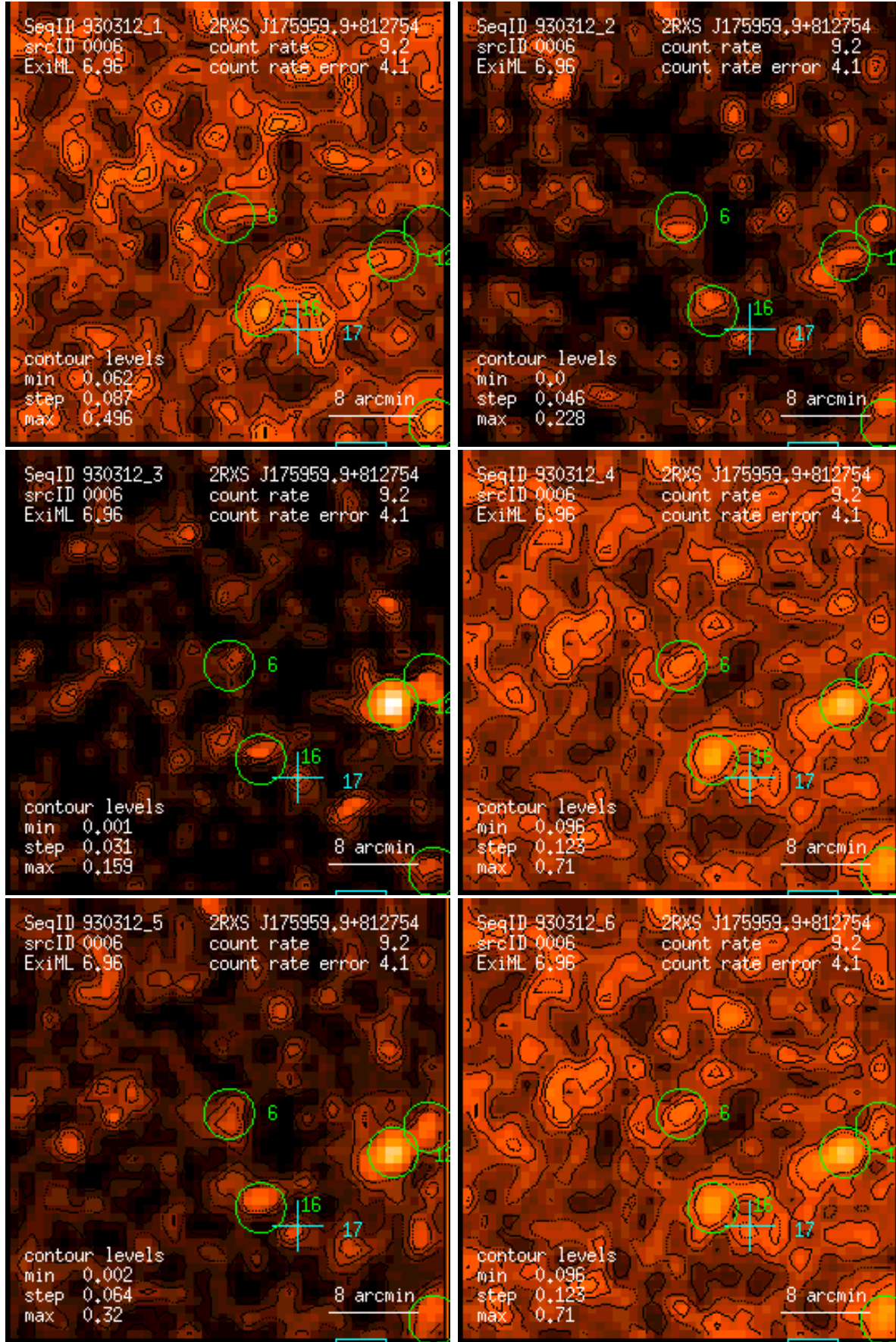
Figure 6: RASS 930312: detection 0006: band rate images, Gaussian filter: (1) PSPC channels 11 – 41, (2) 52 – 90, (3) 91 – 201, (4) 11 – 235, (5) 52 – 201, (6) 11 – 201. Broad band rates in counts/ks. Band rate contour levels in counts/ks/arcmin 2 .
