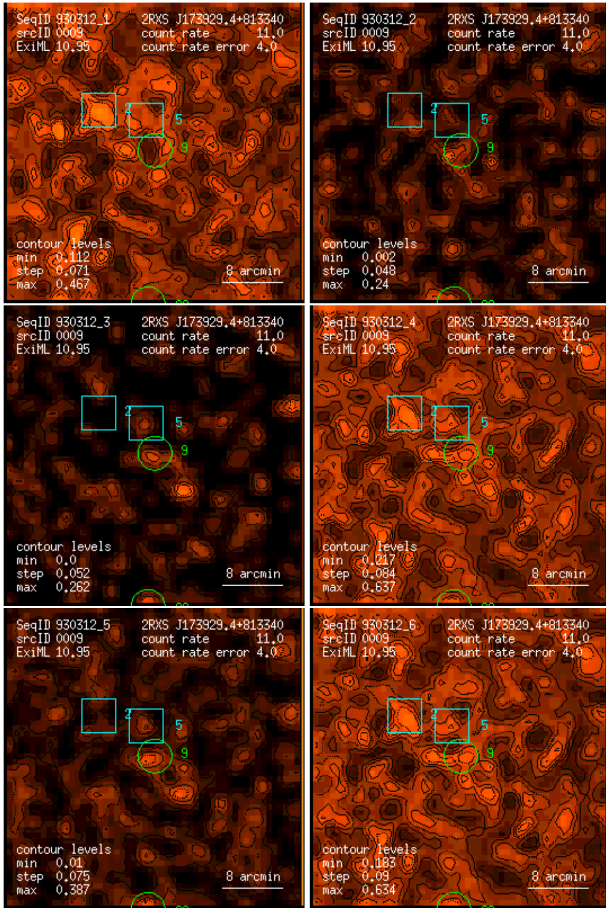
Figure 9: RASS 930312: detection 0009: band rate images, Gaussian filter: (1) PSPC channels 11 – 41, (2) 52 – 90, (3) 91 – 201, (4) 11 – 235, (5) 52 – 201, (6) 11 – 201. Broad band rates in counts/ks. Band rate contour levels in counts/ks/arcmin 2 .
