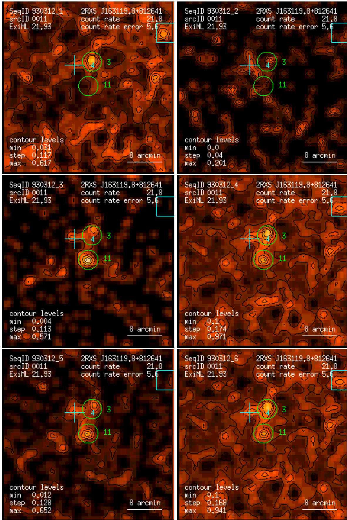
Figure 11: RASS 930312: detection 0011: band rate images, Gaussian filter: (1) PSPC channels 11 – 41, (2) 52 – 90, (3) 91 – 201, (4) 11 – 235, (5) 52 – 201, (6) 11 – 201. Broad band rates in counts/ks. Band rate contour levels in counts/ks/arcmin 2 .
