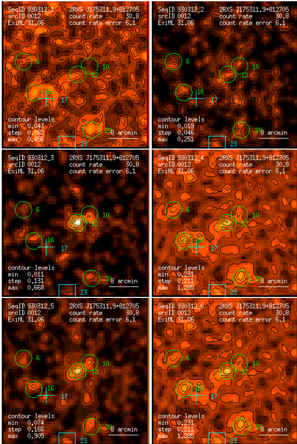
Figure 12: RASS 930312: detection 0012: band rate images, Gaussian filter: (1) PSPC channels 11 – 41, (2) 52 – 90, (3) 91 – 201, (4) 11 – 235, (5) 52 – 201, (6) 11 – 201. Broad band rates in counts/ks. Band rate contour levels in counts/ks/arcmin 2 .
