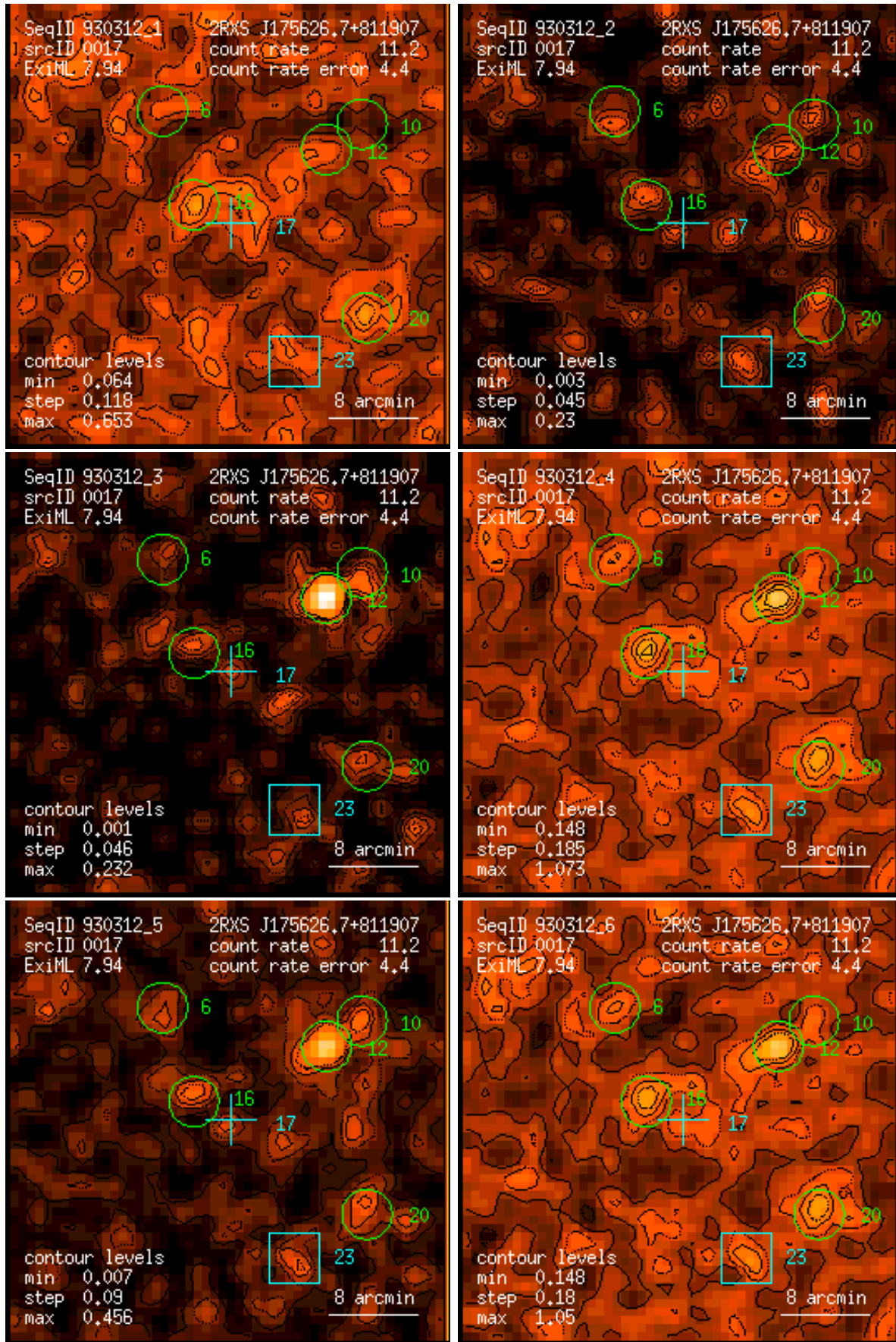
Figure 17: RASS 930312: detection 0017: band rate images, Gaussian filter: (1) PSPC channels 11 – 41, (2) 52 – 90, (3) 91 – 201, (4) 11 – 235, (5) 52 – 201, (6) 11 – 201. Broad band rates in counts/ks. Band rate contour levels in counts/ks/arcmin 2 .
