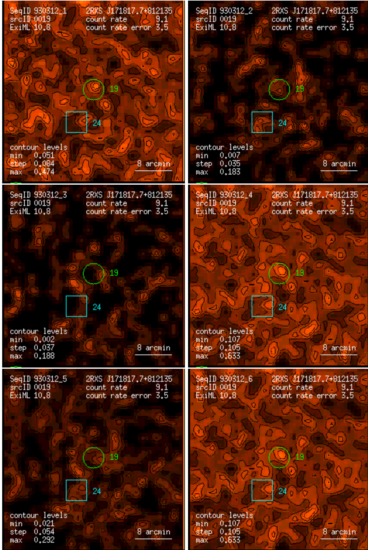
Figure 19: RASS 930312: detection 0019: band rate images, Gaussian filter: (1) PSPC channels 11 – 41, (2) 52 – 90, (3) 91 – 201, (4) 11 – 235, (5) 52 – 201, (6) 11 – 201. Broad band rates in counts/ks. Band rate contour levels in counts/ks/arcmin 2 .
