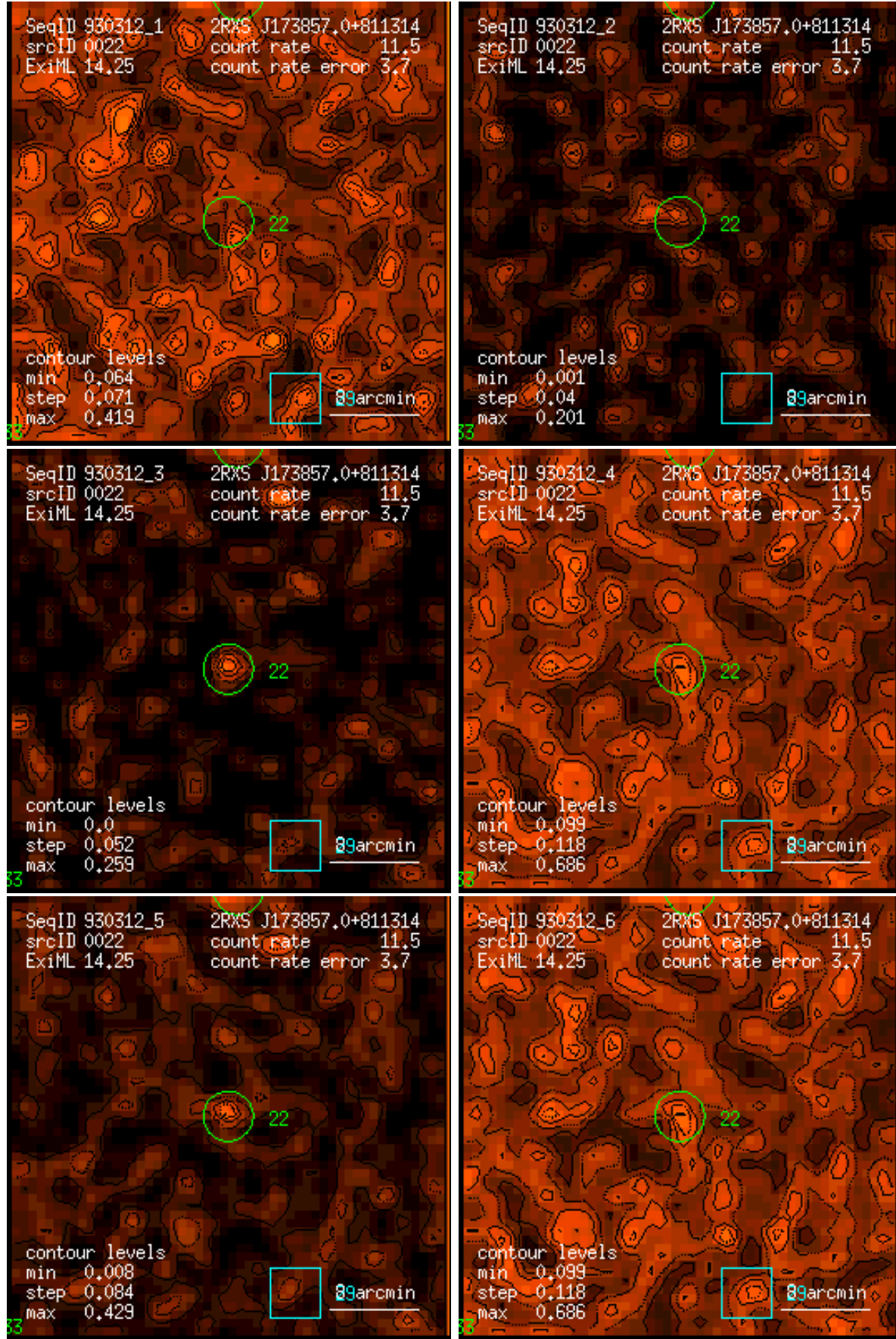
Figure 22: RASS 930312: detection 0022: band rate images, Gaussian filter: (1) PSPC channels 11 – 41, (2) 52 – 90, (3) 91 – 201, (4) 11 – 235, (5) 52 – 201, (6) 11 – 201. Broad band rates in counts/ks. Band rate contour levels in counts/ks/arcmin 2 .
