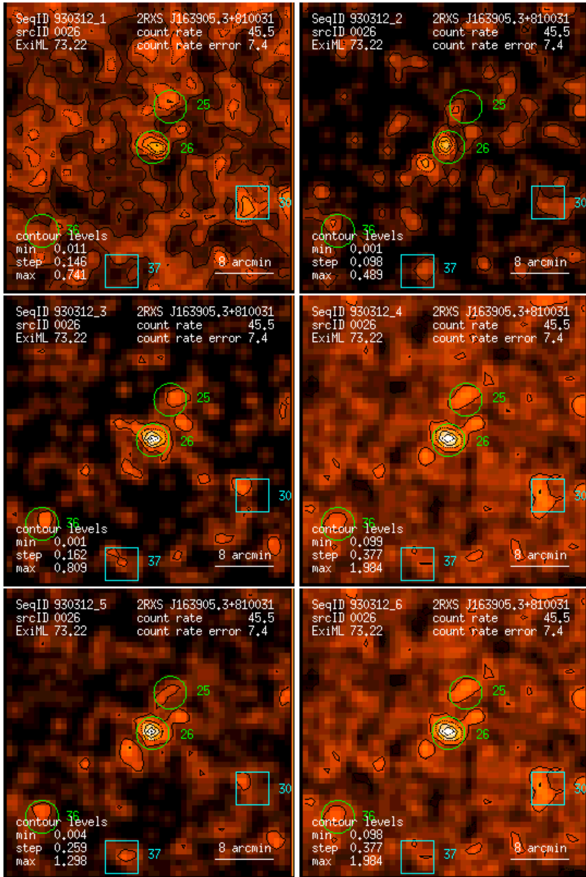
Figure 26: RASS 930312: detection 0026: band rate images, Gaussian filter: (1) PSPC channels 11 – 41, (2) 52 – 90, (3) 91 – 201, (4) 11 – 235, (5) 52 – 201, (6) 11 – 201. Broad band rates in counts/ks. Band rate contour levels in counts/ks/arcmin 2 .
