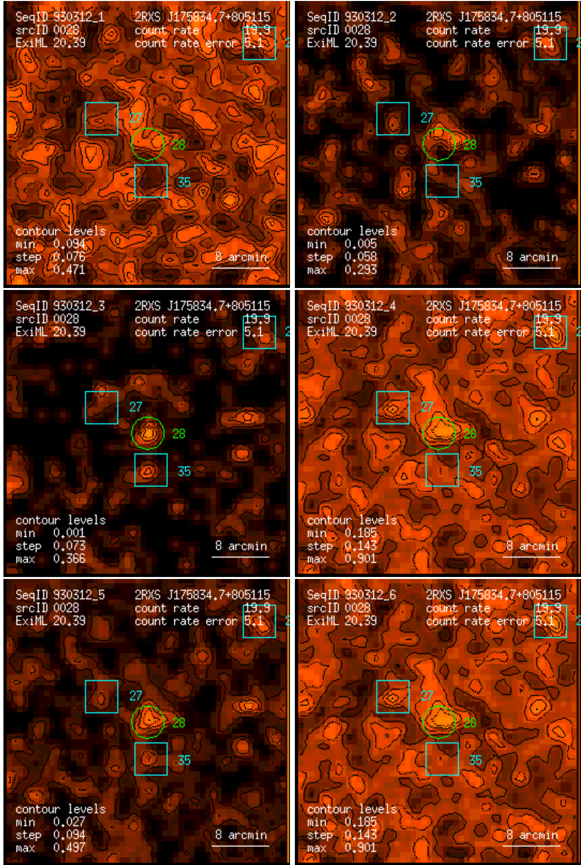
Figure 28: RASS 930312: detection 0028: band rate images, Gaussian filter: (1) PSPC channels 11 – 41, (2) 52 – 90, (3) 91 – 201, (4) 11 – 235, (5) 52 – 201, (6) 11 – 201. Broad band rates in counts/ks. Band rate contour levels in counts/ks/arcmin 2 .
