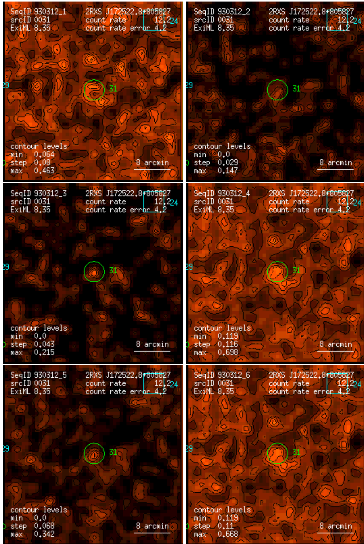
Figure 31: RASS 930312: detection 0031: band rate images, Gaussian filter: (1) PSPC channels 11 – 41, (2) 52 – 90, (3) 91 – 201, (4) 11 – 235, (5) 52 – 201, (6) 11 – 201. Broad band rates in counts/ks. Band rate contour levels in counts/ks/arcmin 2 .
