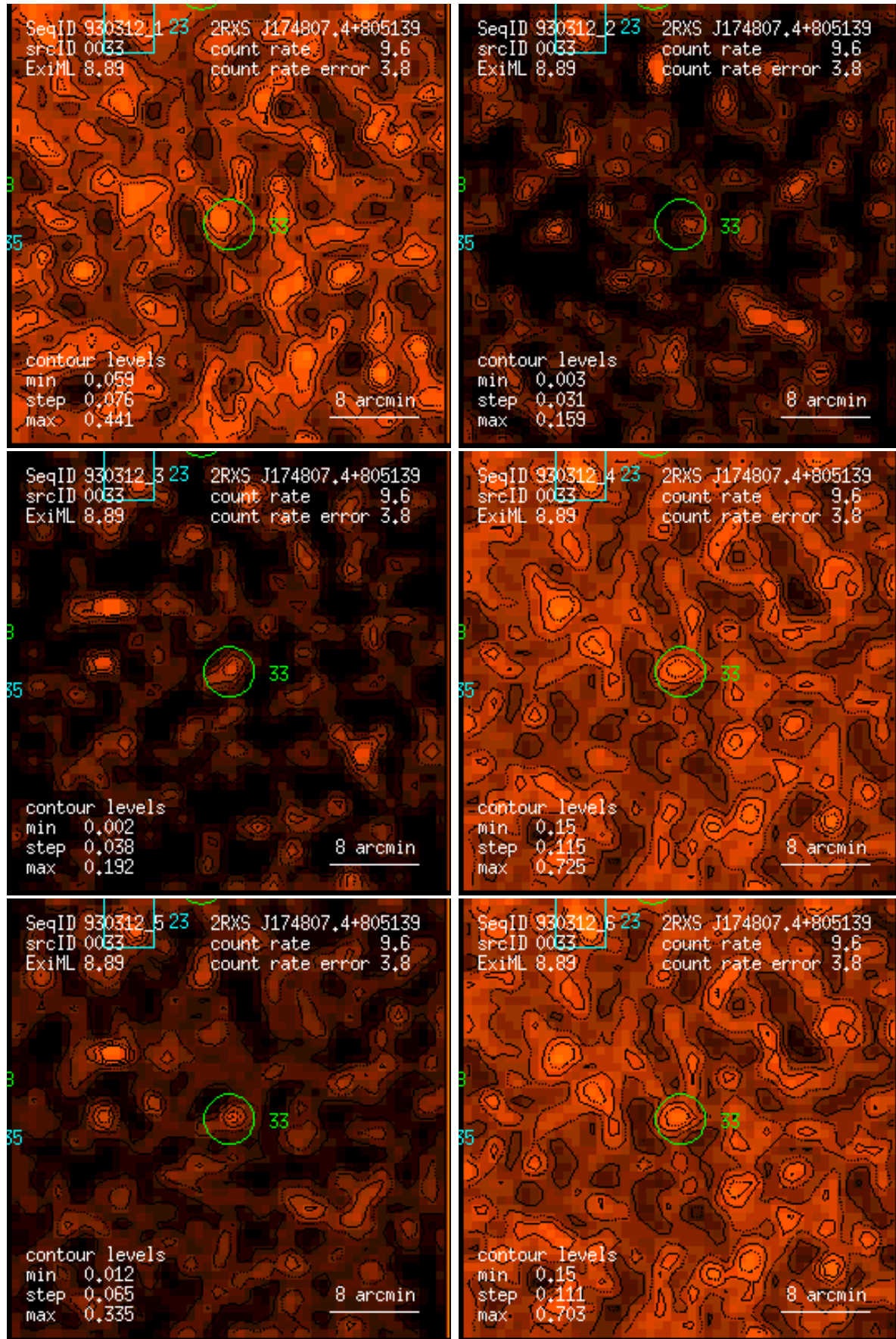
Figure 33: RASS 930312: detection 0033: band rate images, Gaussian filter: (1) PSPC channels 11 – 41, (2) 52 – 90, (3) 91 – 201, (4) 11 – 235, (5) 52 – 201, (6) 11 – 201. Broad band rates in counts/ks. Band rate contour levels in counts/ks/arcmin 2 .
