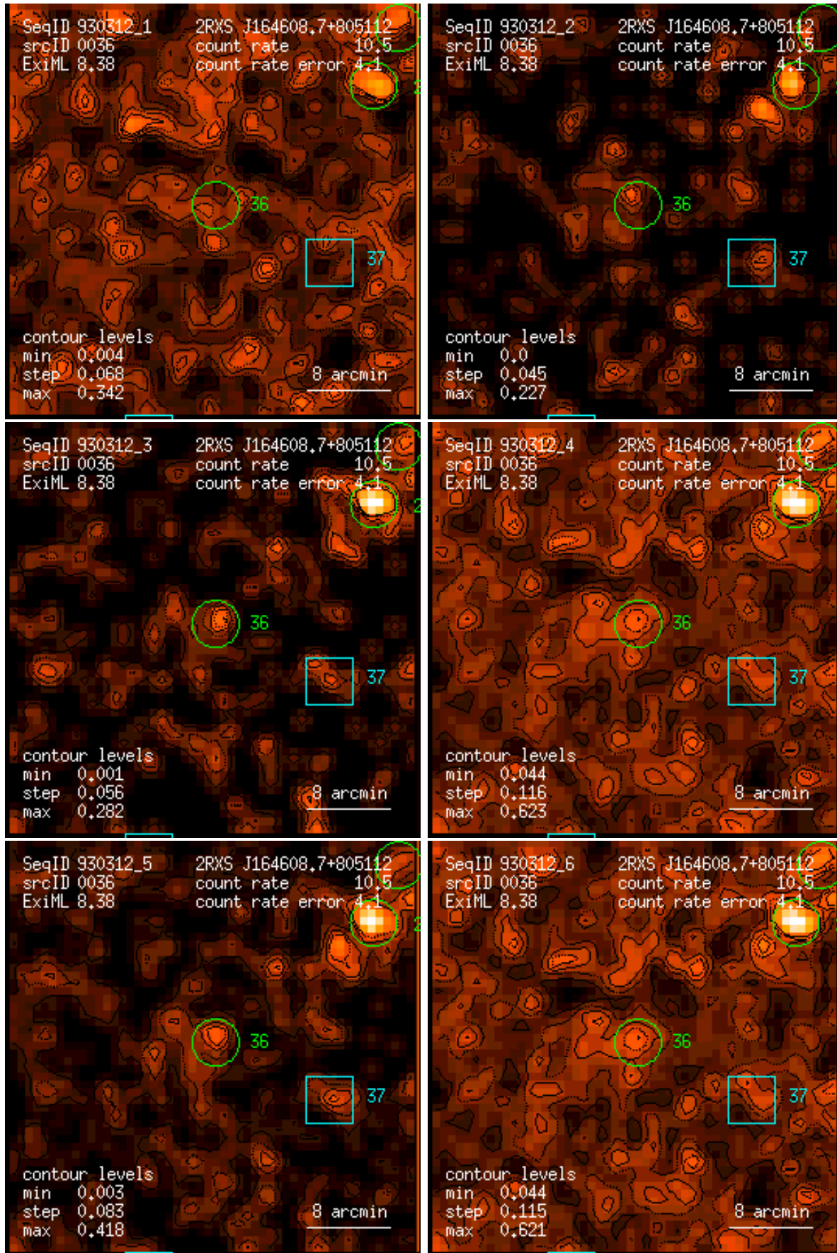
Figure 36: RASS 930312: detection 0036: band rate images, Gaussian filter: (1) PSPC channels 11 – 41, (2) 52 – 90, (3) 91 – 201, (4) 11 – 235, (5) 52 – 201, (6) 11 – 201. Broad band rates in counts/ks. Band rate contour levels in counts/ks/arcmin 2 .
