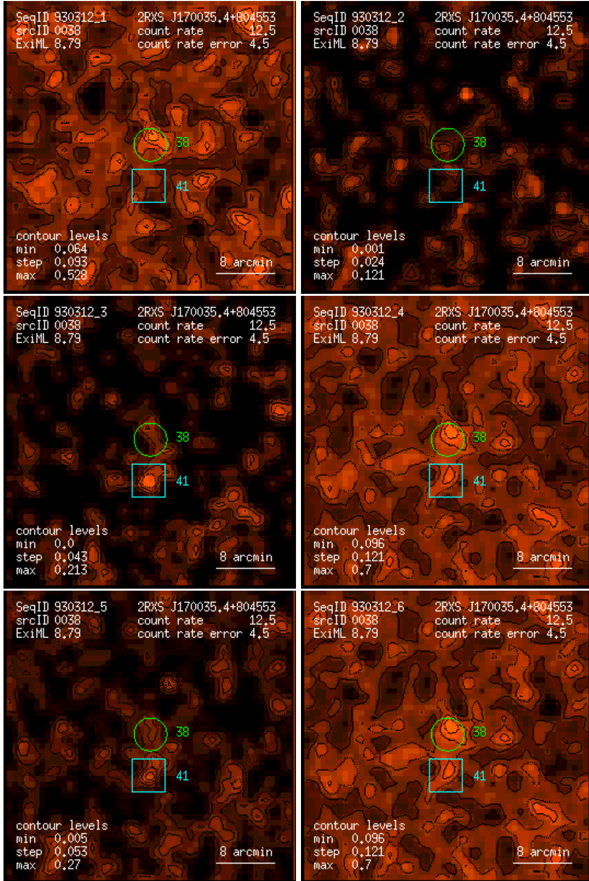
Figure 38: RASS 930312: detection 0038: band rate images, Gaussian filter: (1) PSPC channels 11 – 41, (2) 52 – 90, (3) 91 – 201, (4) 11 – 235, (5) 52 – 201, (6) 11 – 201. Broad band rates in counts/ks. Band rate contour levels in counts/ks/arcmin 2 .
